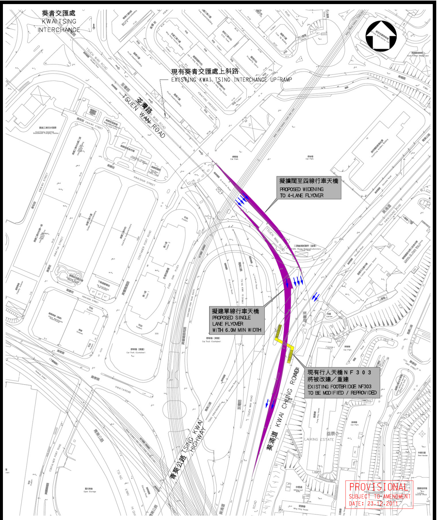
Project Title: Flyover from Kwai Tsing Interchange Up-ramp to Kwai Chung Road Figure 2: Road Layout Plan (Option 2) (Extracted from the Drawing 1.2 of the Project Profile)
