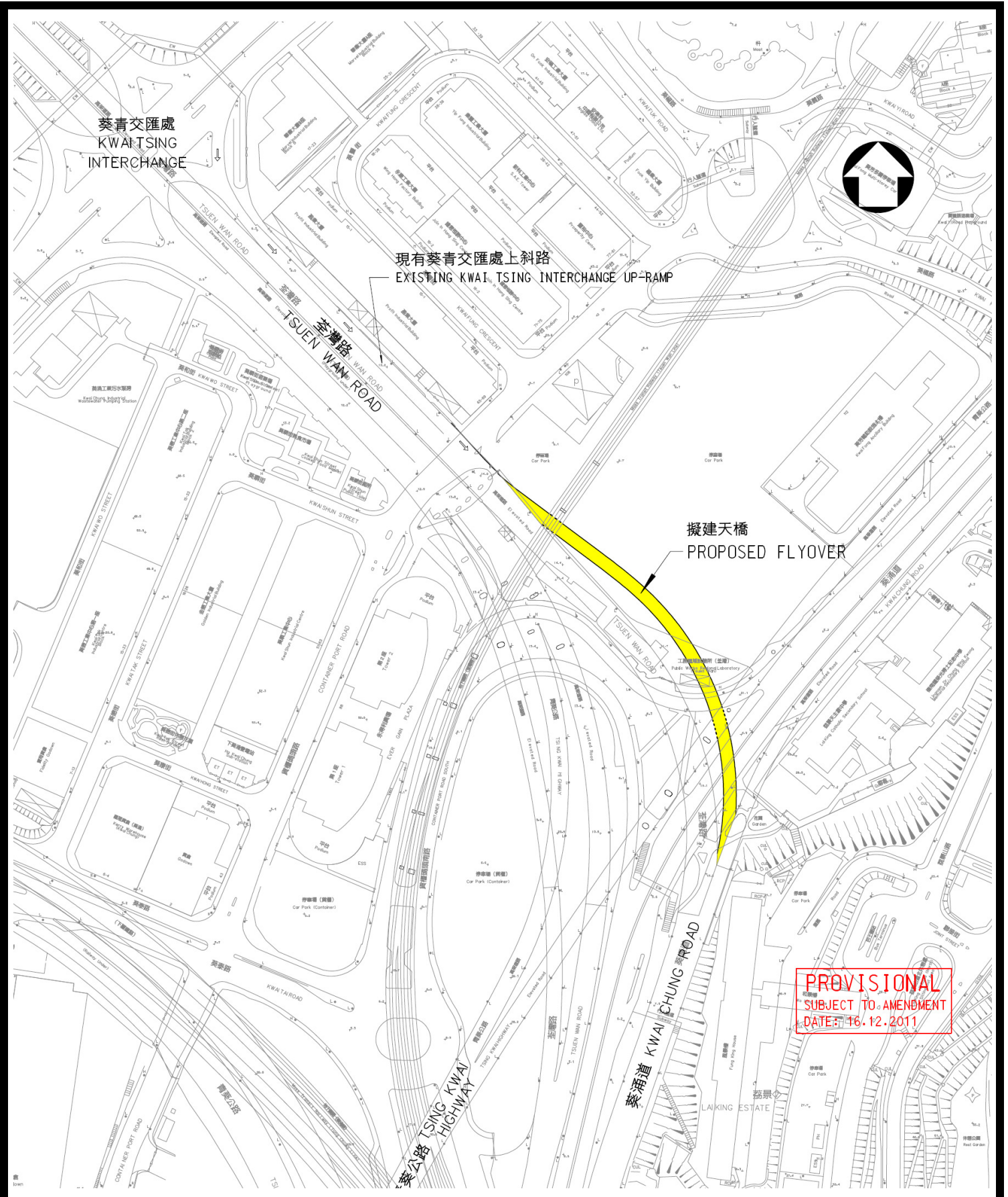
Project Title: Flyover from Kwai Tsing Interchange Up-ramp to Kwai Chung Road Figure 1: Road Layout Plan (Option 1) (Extracted from the Drawing 1.1 of the Project Profile)
