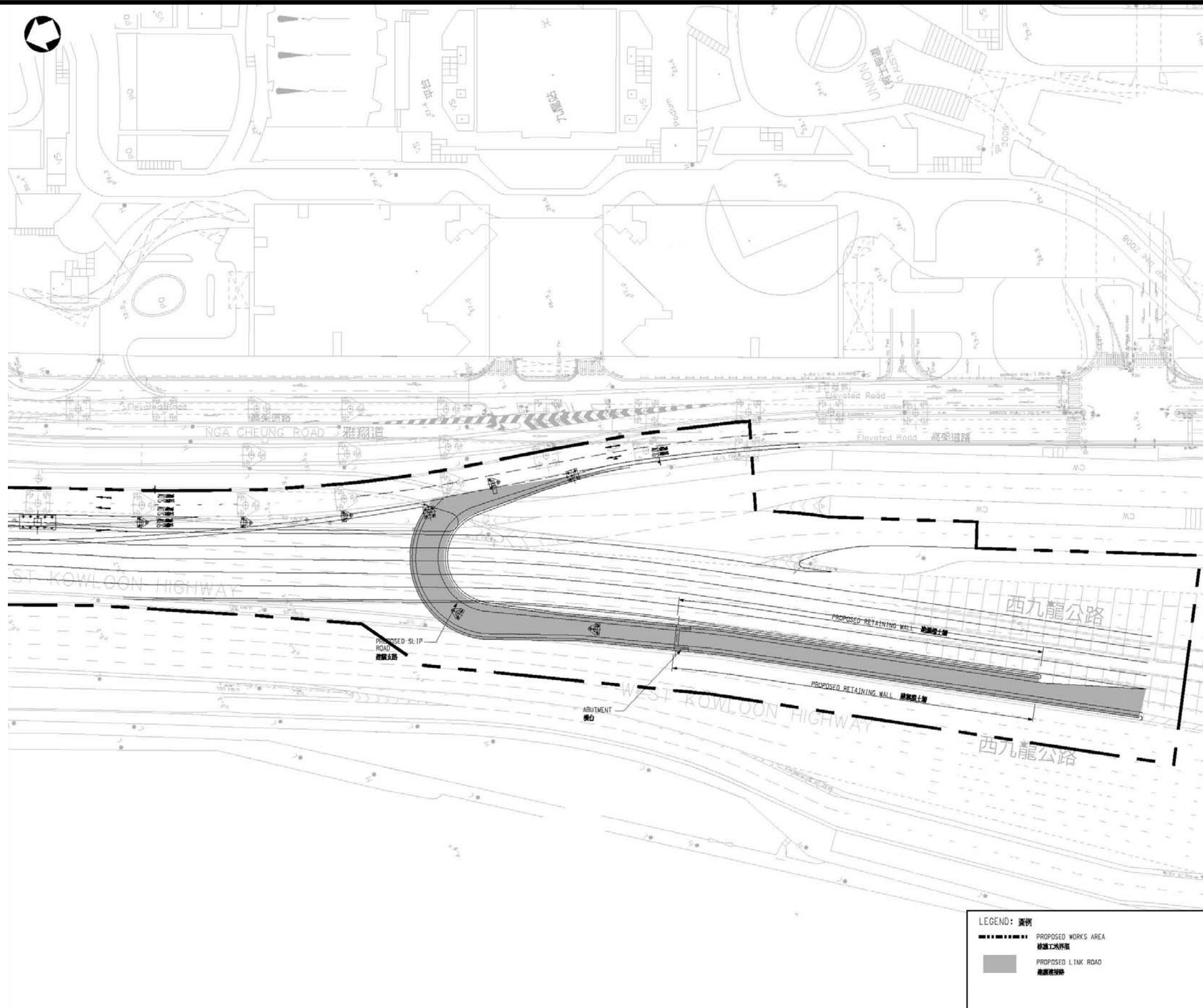
Figure 6: NEW LINK ROAD FROM NGA CHEUNG ROAD TO WEST HARBOUR CROSSING – SCHEME I ROAD LAYOUT PLAN
