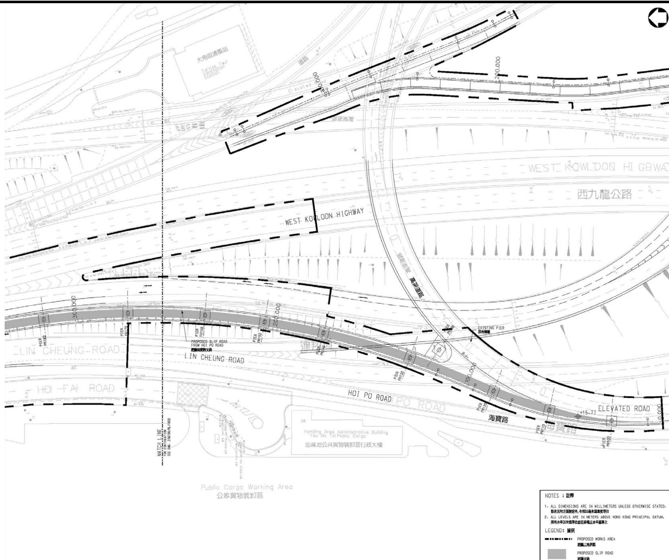
Figure 2: PROPOSED SLIP ROAD FROM HOI PO ROAD TO WEST KOWLOON HIGHWAY – SCHEME H (PART A) ROAD LAYOUT PLAN (SHEET 1 OF 3) 圖二: 建議由海寶路至西九龍公路的新支路 - 計劃H(A部份)道路平面佈置圖(頁一)
