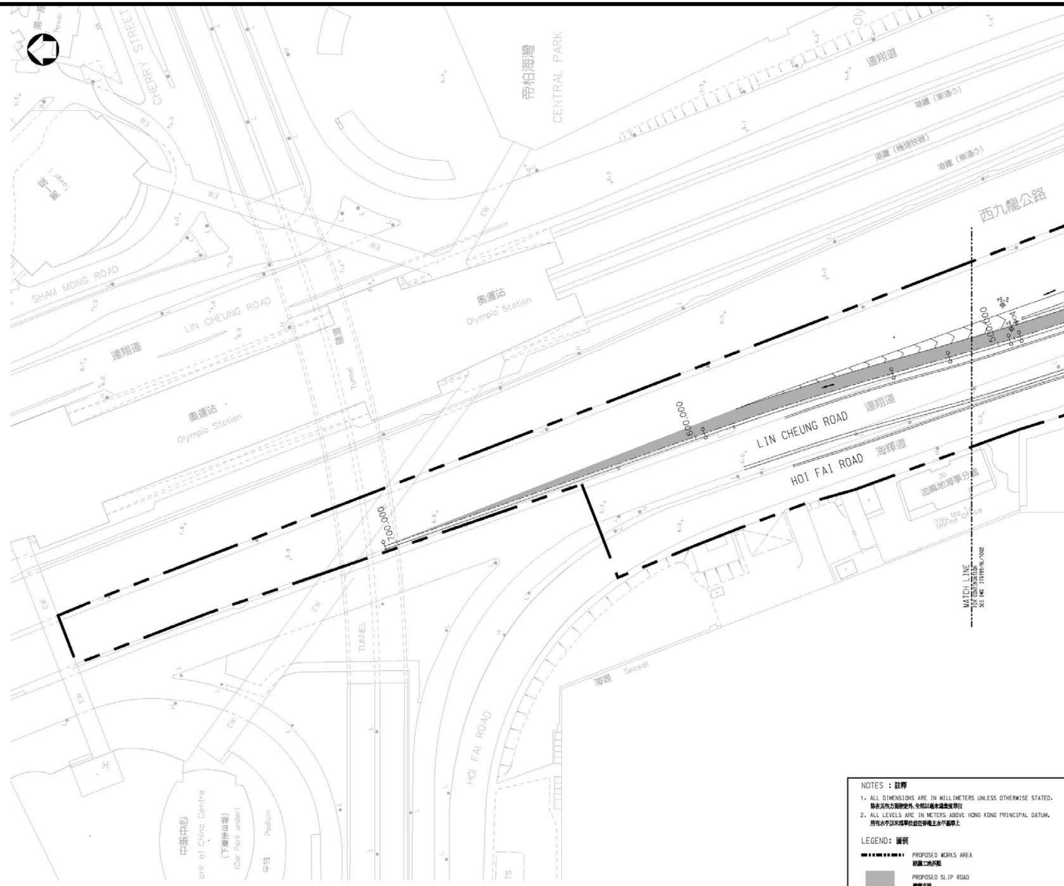
Figure 4: PROPOSED SLIP ROAD FROM HOI PO ROAD TO WEST KOWLOON HIGHWAY – SCHEME H (PART A) ROAD LAYOUT PLAN (SHEET 3 OF 3) 圖 四: 建議由海寶路至西九龍公路的新支路 - 計劃 H (A 部份) 道路平面佈置圖 (頁三)
