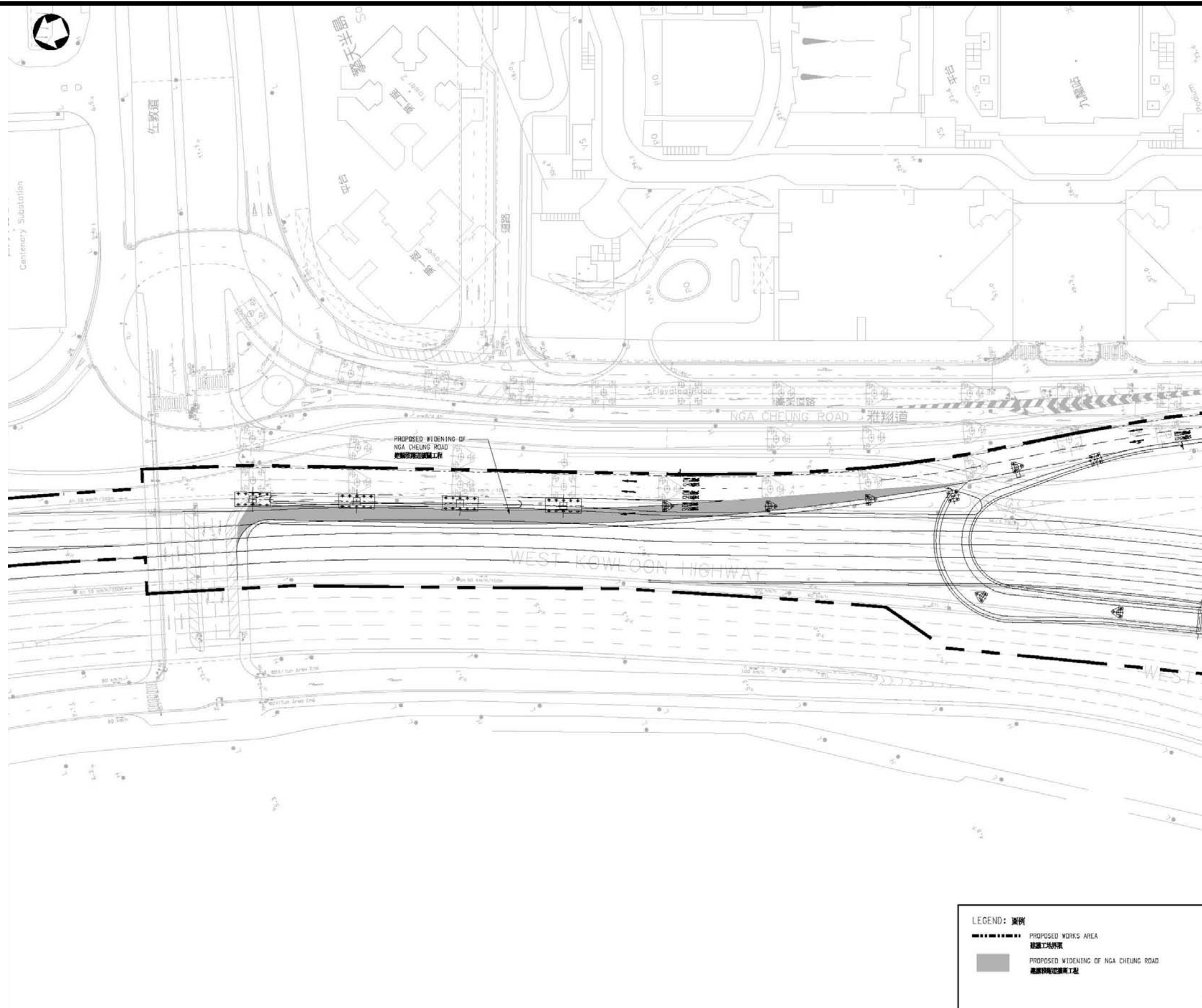
Figure 5: WIDENING OF NGA CHEUNG ROAD – SCHEME H (PART B) ROAD
