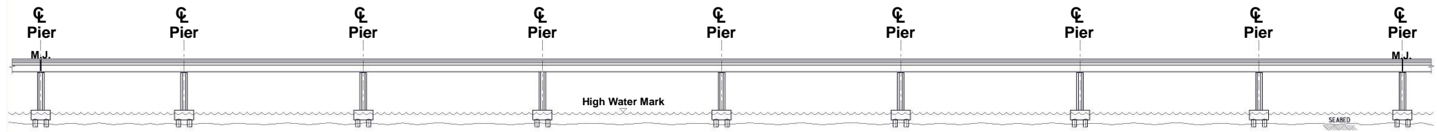
Typical Elevation for Viaducts with Spans up to ~75m without haunches
