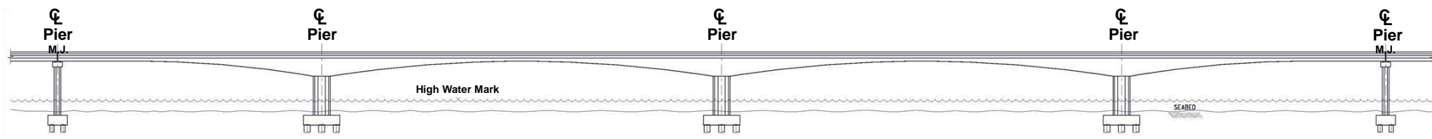
Typical Elevation for Viaducts with Larger Spans of ~100m to ~180m with haunches
