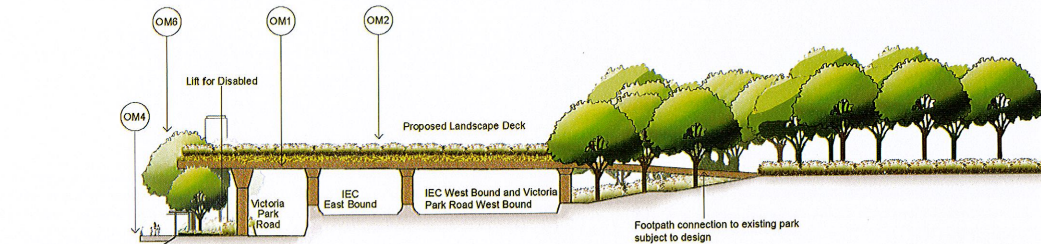
Section F-F
