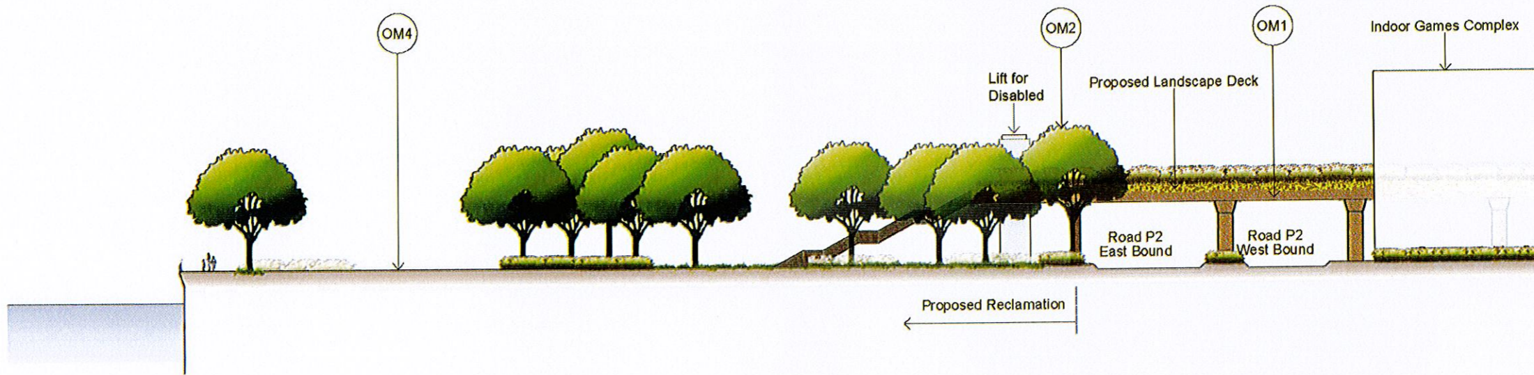
Section E-E
