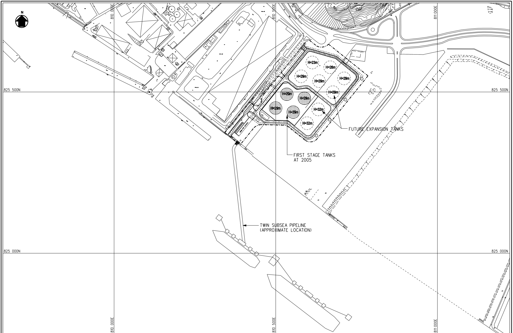
PREVIOUS CONCEPT LAYOUT OF PERMANENT AVIATION FUEL FACILITY TANK FARM AND JETTY WITHIN TUEN MUN AREA 38
