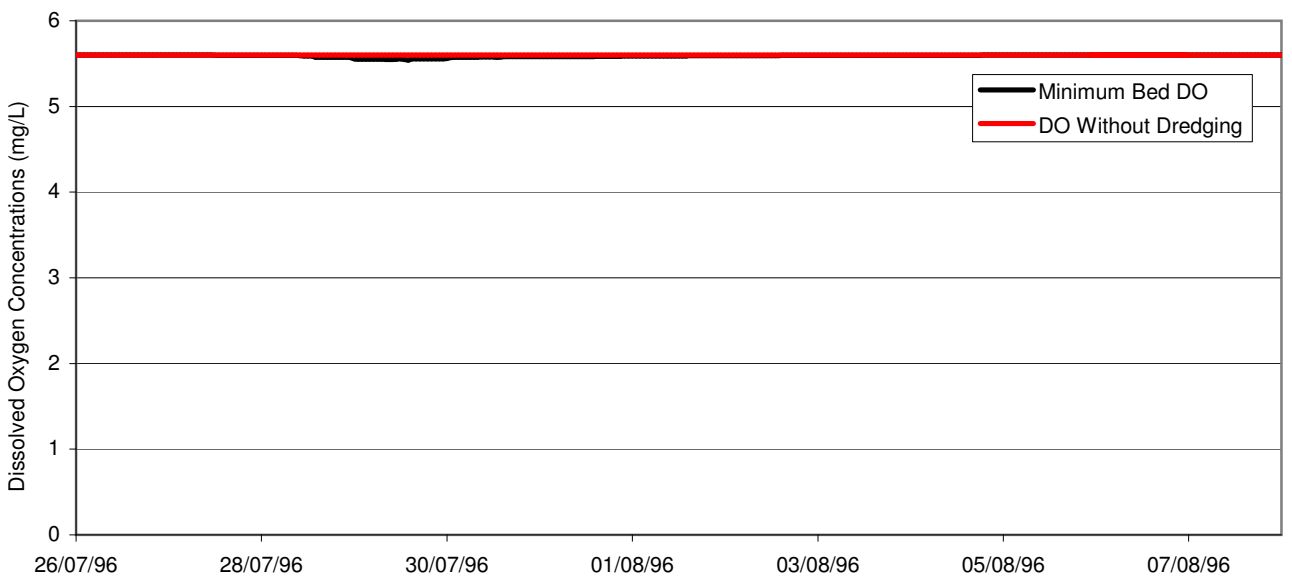
Figure 6.15 Predicted Minimum DO Concentration (mg/L), East of Sha Chau
