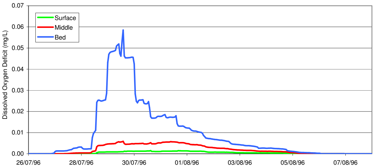
Figure 6.14 Daily Averaged DO Deficit (mg/L) at East of Sha Chau
