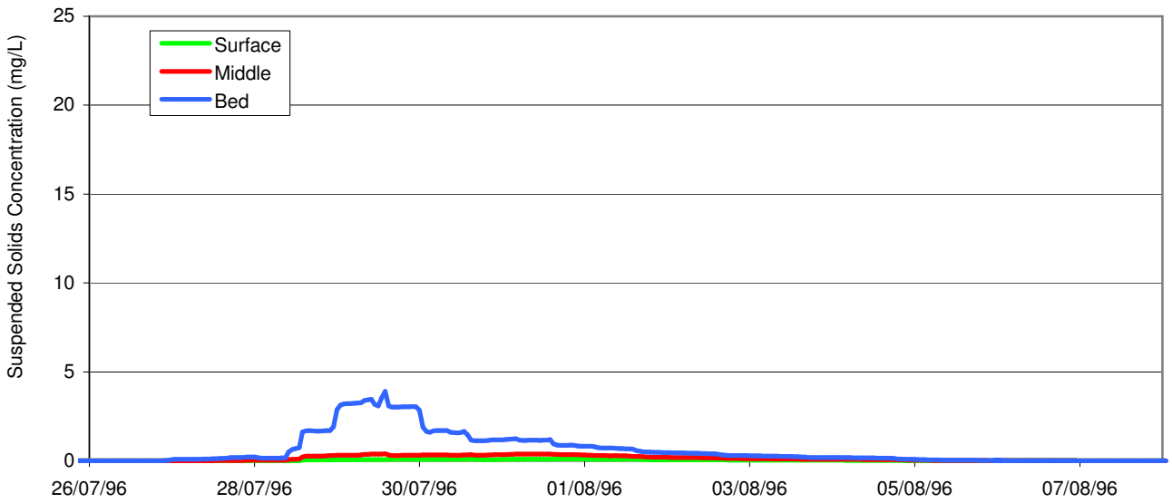
Figure 6.13 Daily Averaged Suspended Solids Concentration, East of Sha Chau
