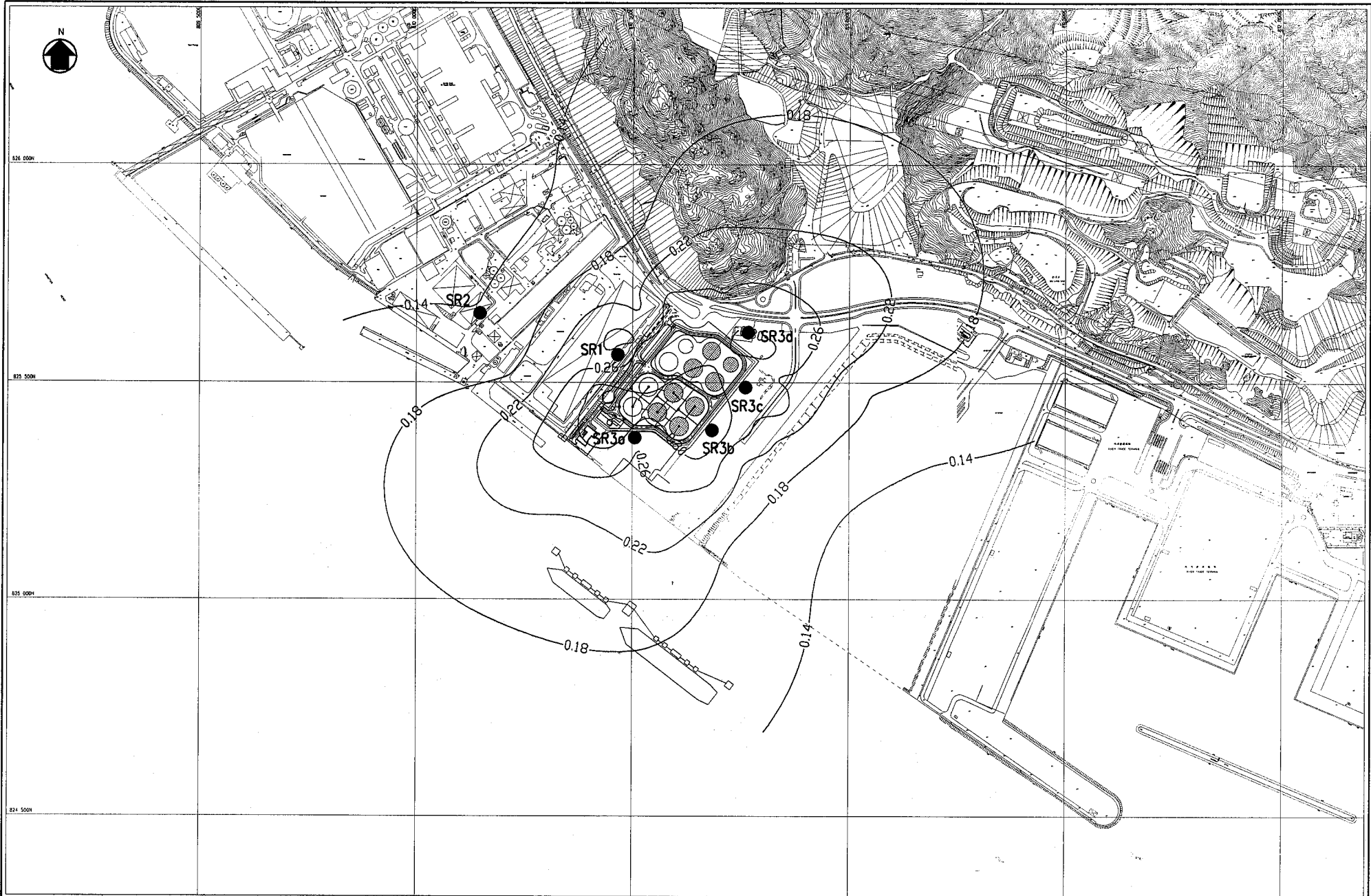
Maximum (5 - second) odour level (OU) plot at 30m above ground (at day-time)
