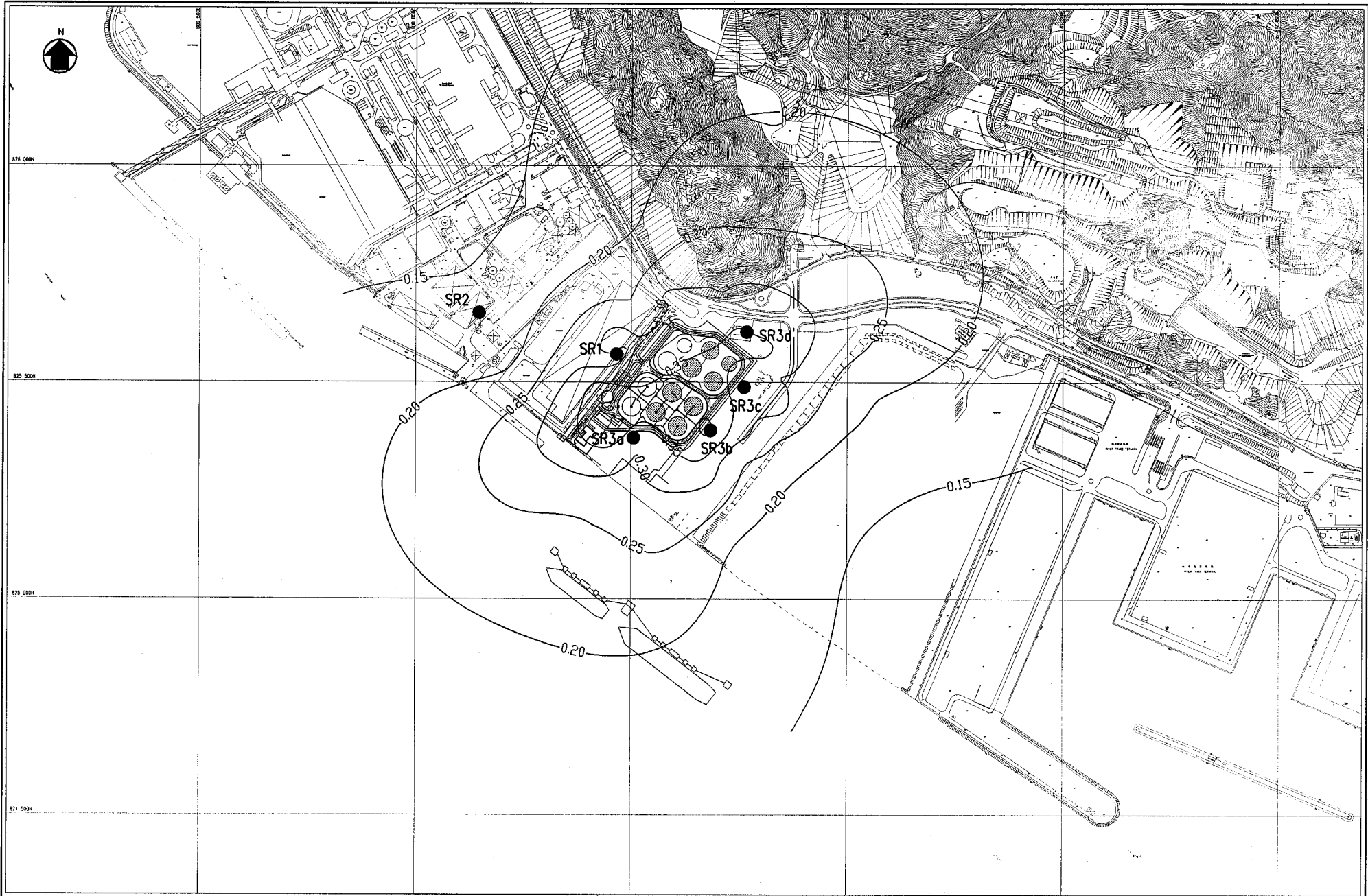
Maximum (5 - second) odour level (OU) plot at 23m above ground (at day-time)
