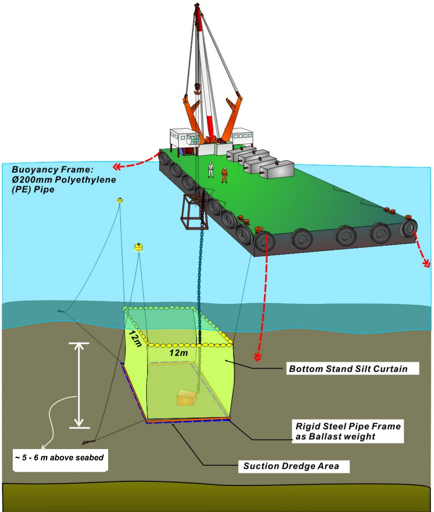
Installation of Fully Enclosed Silt Curtain during the Suction Dredge Operation
