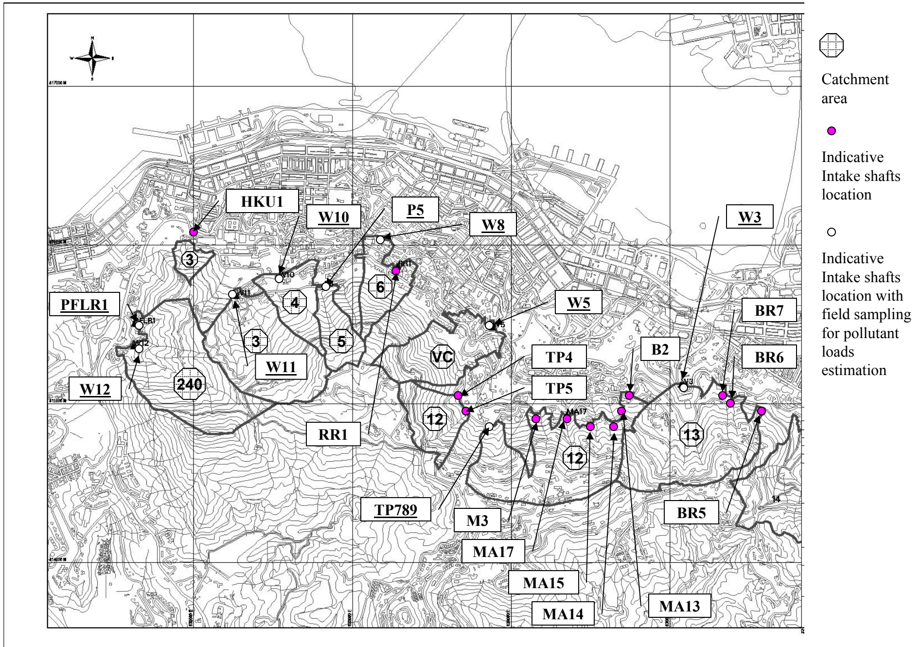
Figure 7.1 Catchment area for the proposed drainage channel (Part 1 of 2)
