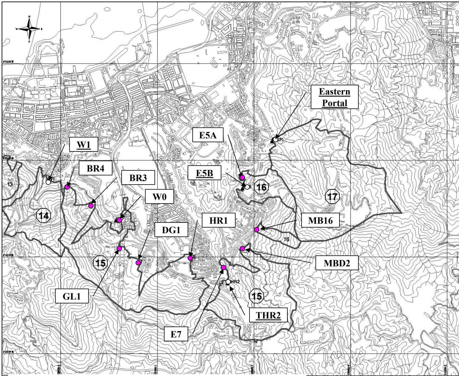
Figure 7.1 Catchment area for the proposed drainage channel (Part 2 of 2)
