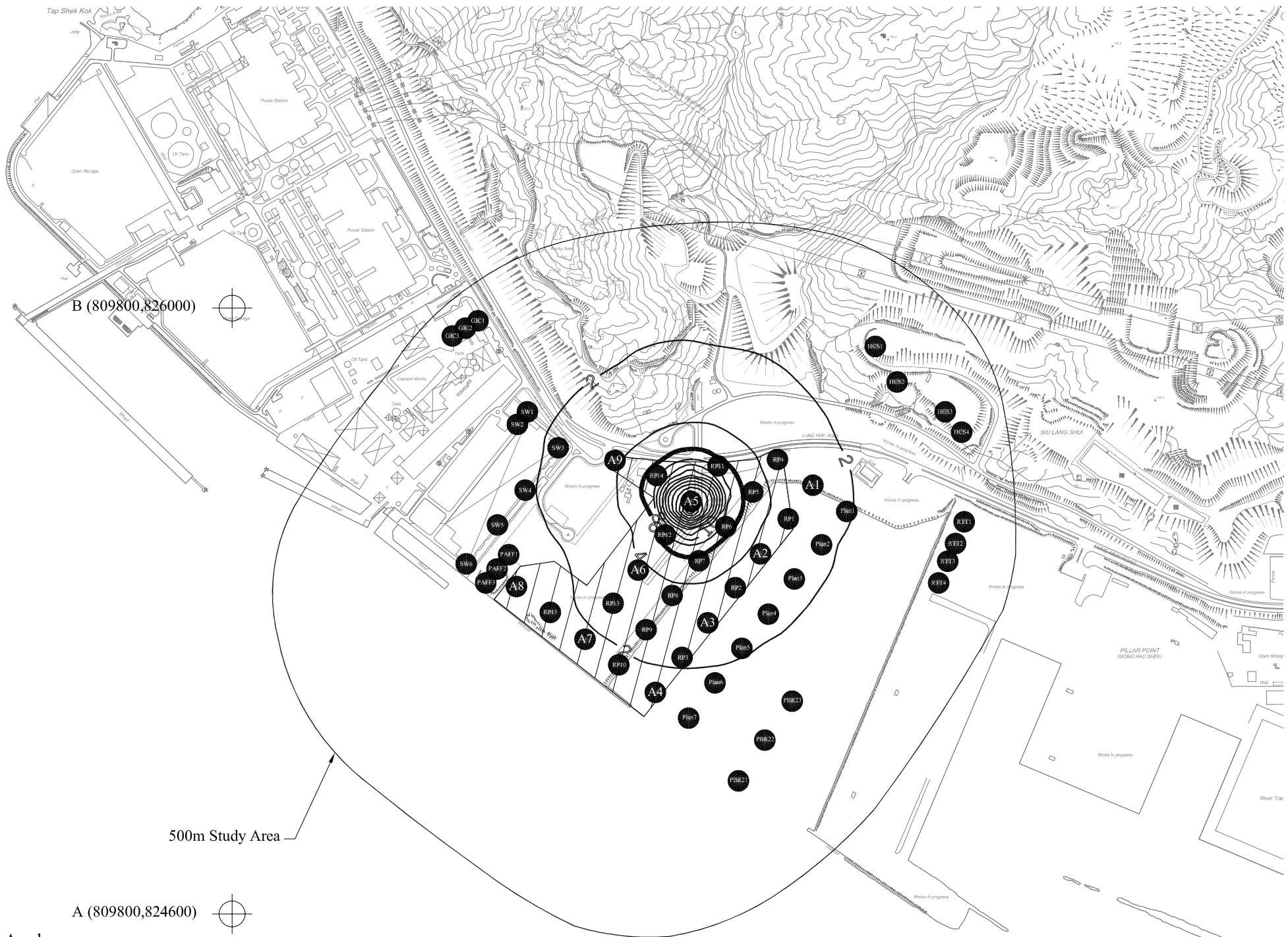
Figure 7-K6 Cumulative 1-hour Ni Concentration ( \mu\text{g}/\text{m}^3 ) at 61.5mPD emitted from Source Location A5 (Mitigated Scenario 2)
