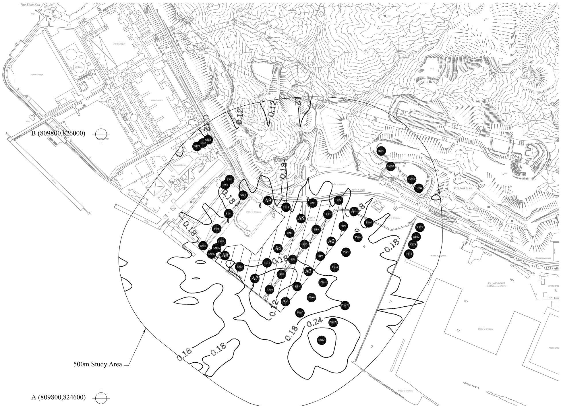
Figure 7-K1 Cumulative 1-hour Ni Concentration ( \mu\text{g}/\text{m}^3 ) at 8.5mPD emitted from Source Location A4 (Mitigated Scenario 2)
