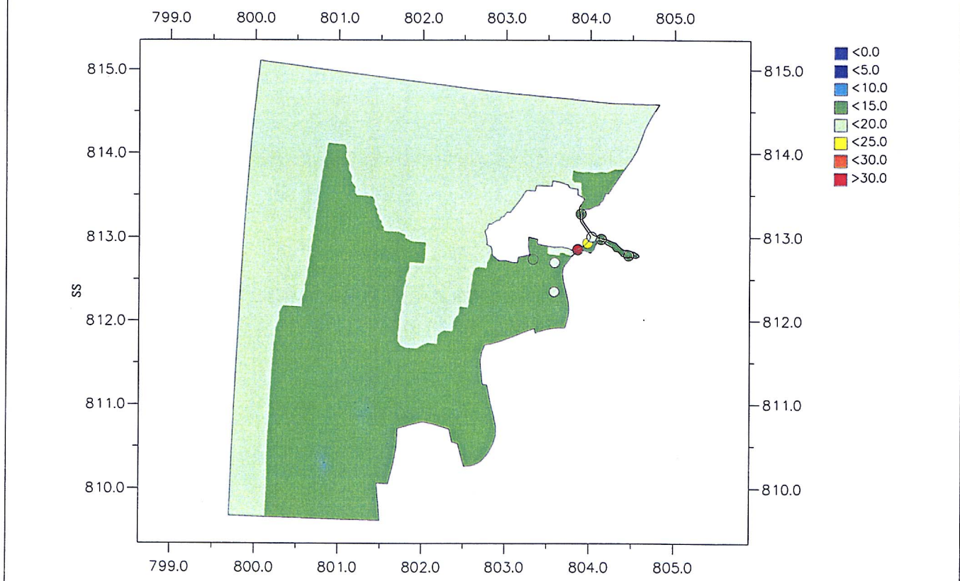
Surface Layer Suspended Solids; Wet Season; Spring Ebb Upper - Fine Grid Regional Model; Lower - Tai O Detailed Model Dots - PPFS Field Data Figure 4D2a
