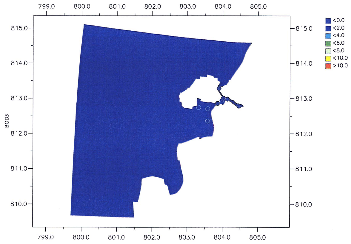
Surface Layer BOD 5 ; Wet Season; Spring Ebb Upper – Fine Grid Regional Model; Lower – Tai O Detailed Model Dots – PPFS Field Data
