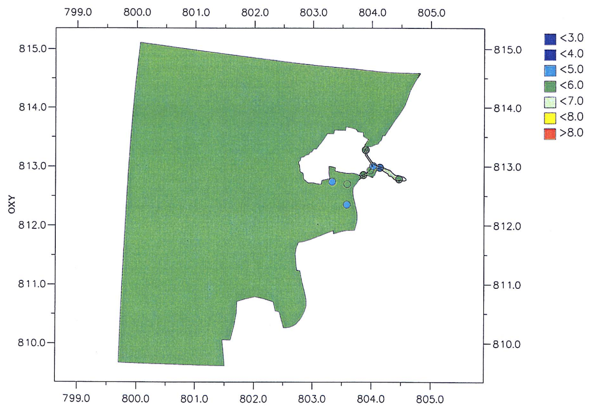
Surface Layer Dissolved Oxygen; Wet Season; Spring Ebb Upper - Fine Grid Regional Model; Lower - Tai O Detailed Model Dots - PPFS Field Data
