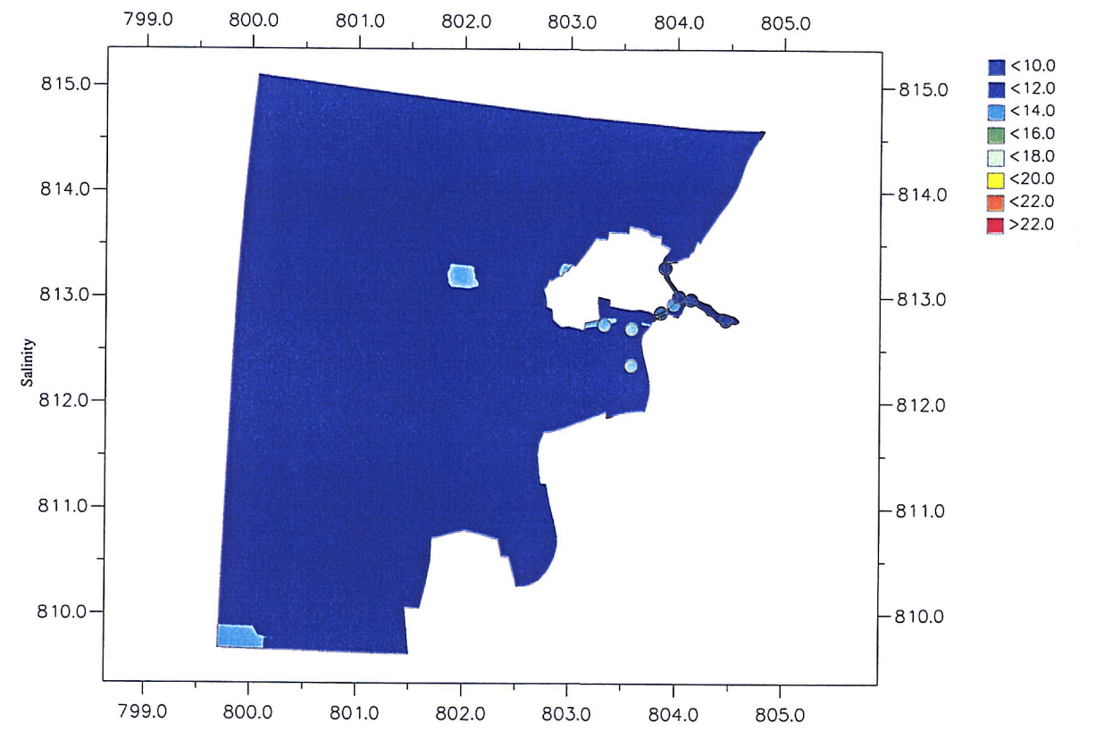
Surface Layer Salinity; Wet Season; Neap Flood Upper - Fine Grid Regional Model; Lower - Tai O Detailed Model Dots - PPFS Field Data
