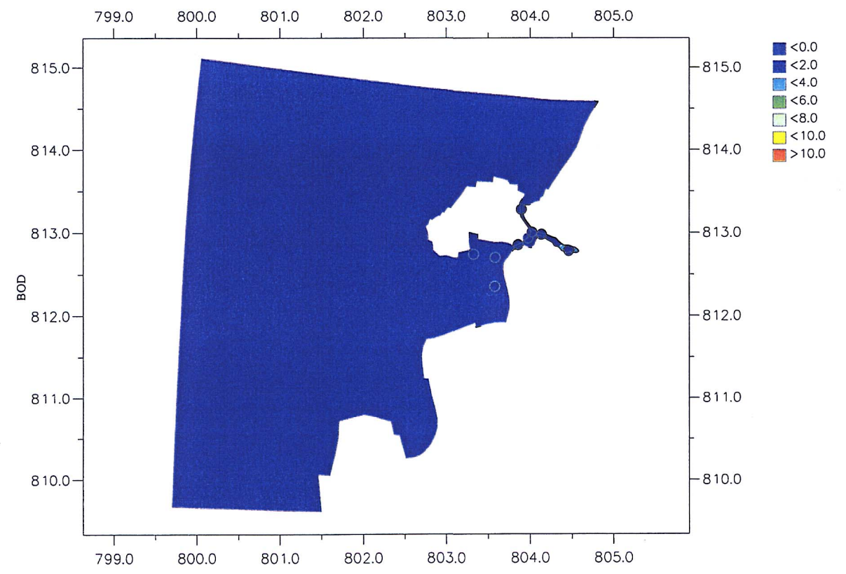
Surface Layer BOD; Wet Season; Neap Flood Upper – Fine Grid Regional Model; Lower – Tai O Detailed Model Dots – PPFS Field Data
