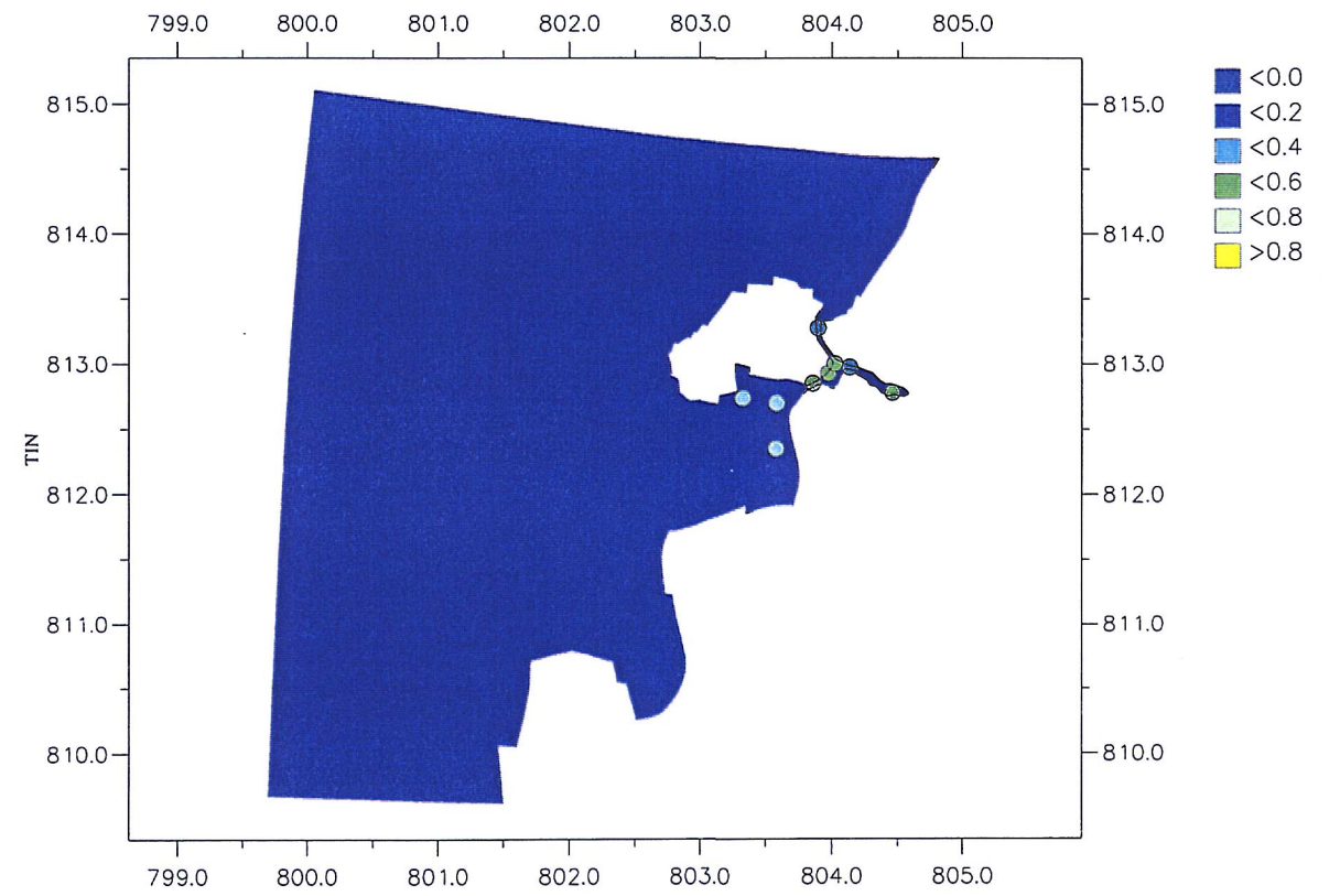
Surface Layer Total Inorganic Nitrogen; Wet Season; Neap Flood Upper - Fine Grid Regional Model; Lower - Tai O Detailed Model Dots - PPFS Field Data
