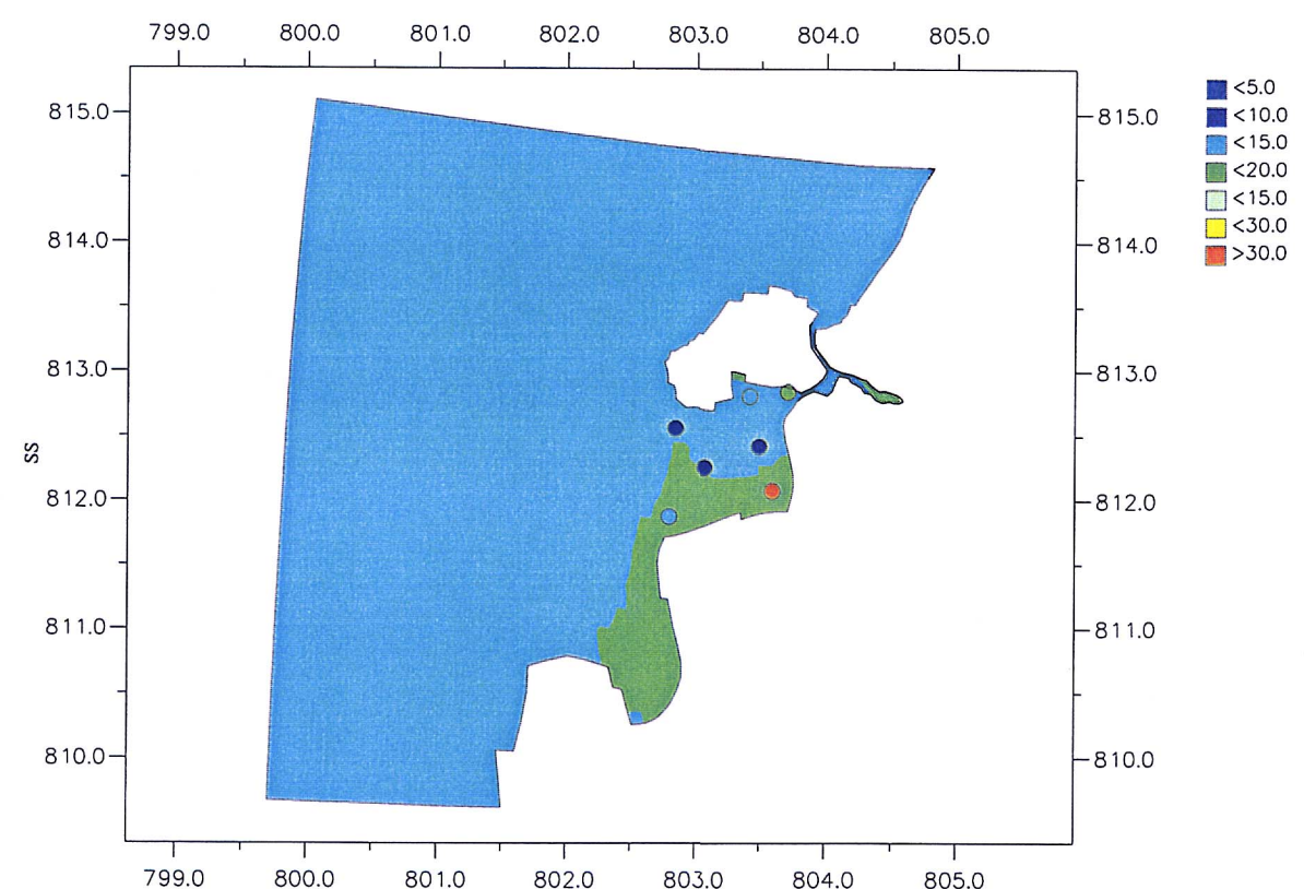
Surface Layer Suspended Solids; Dry Season; Low Water Upper - Fine Grid Regional Model; Lower - Tai O Detailed Model Dots - Tai O Boat Anchorage Field Data
