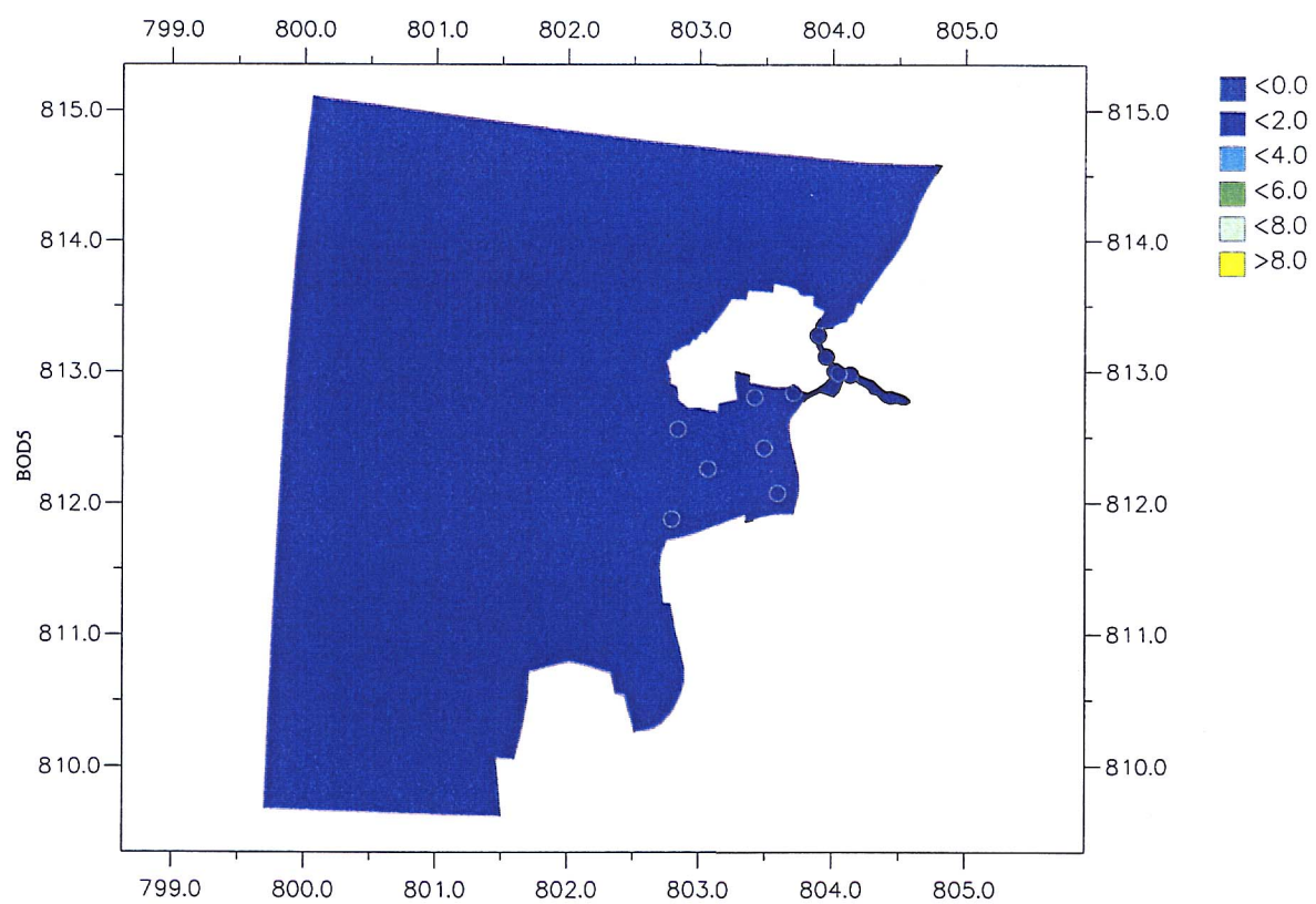
Surface Layer BOD; Dry Season; Low Water Upper – Fine Grid Regional Model; Lower – Tai O Detailed Model Dots at Tai O Bay – Tai O Boat Anchorage Field Data
