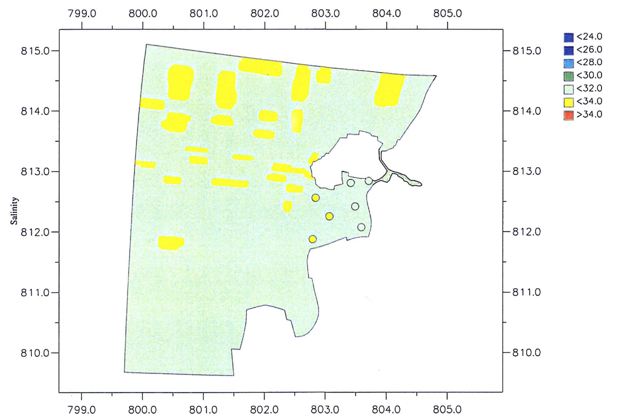
Surface Layer Salinity; Dry Season; Low Water Upper - Fine Grid Regional Model; Lower - Tai O Detailed Model Dots - Tai O Boat Anchorage Field Data
