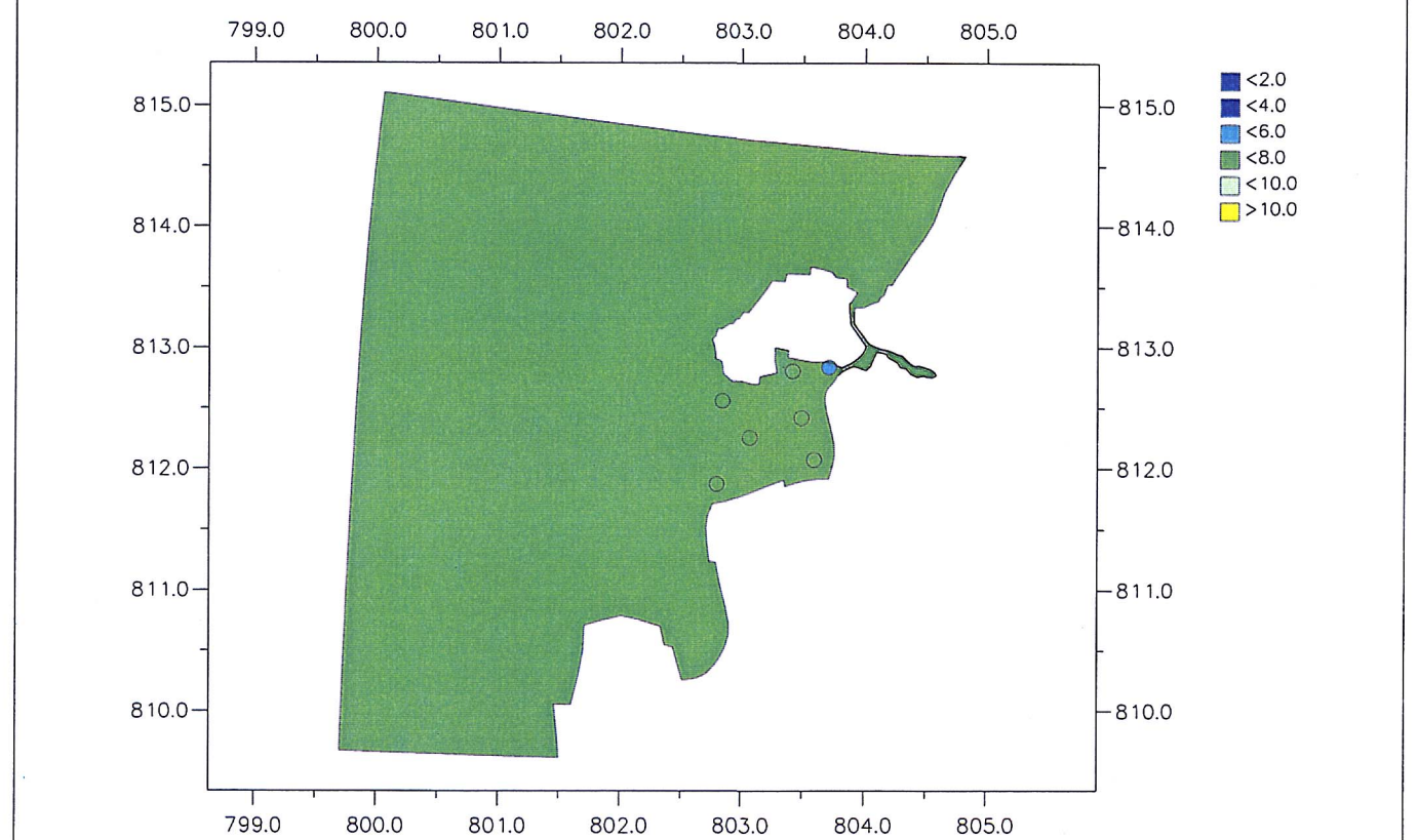
Surface Layer Dissolved Oxygen; Dry Season; Low Water Upper - Fine Grid Regional Model; Lower - Tai O Detailed Model Dots - Tai O Boat Anchorage Field Data
