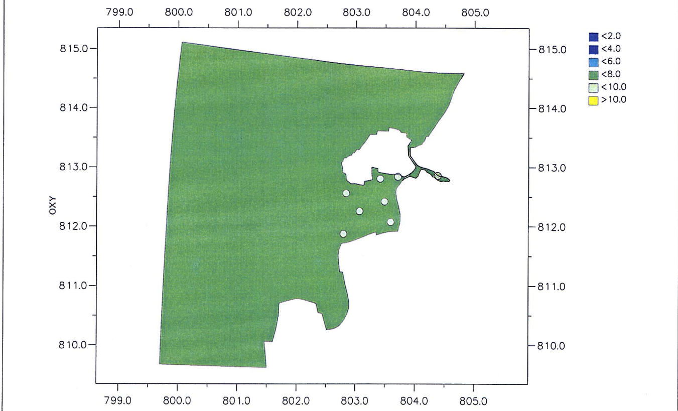
Surface Layer Dissolved Oxygen; Dry Season; High Water Upper - Fine Grid Regional Model; Lower - Tai O Detailed Model Dots - Tai O Boat Anchorage Field Data
