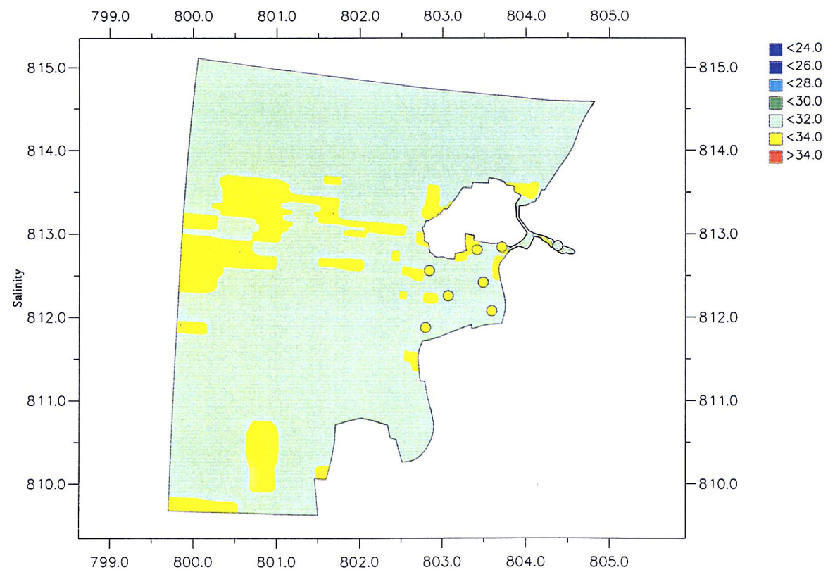
Surface Layer Salinity; Dry Season; High Water Upper - Fine Grid Regional Model; Lower - Tai O Detailed Model; Dots - Tai O Boat Anchorage Field Data
