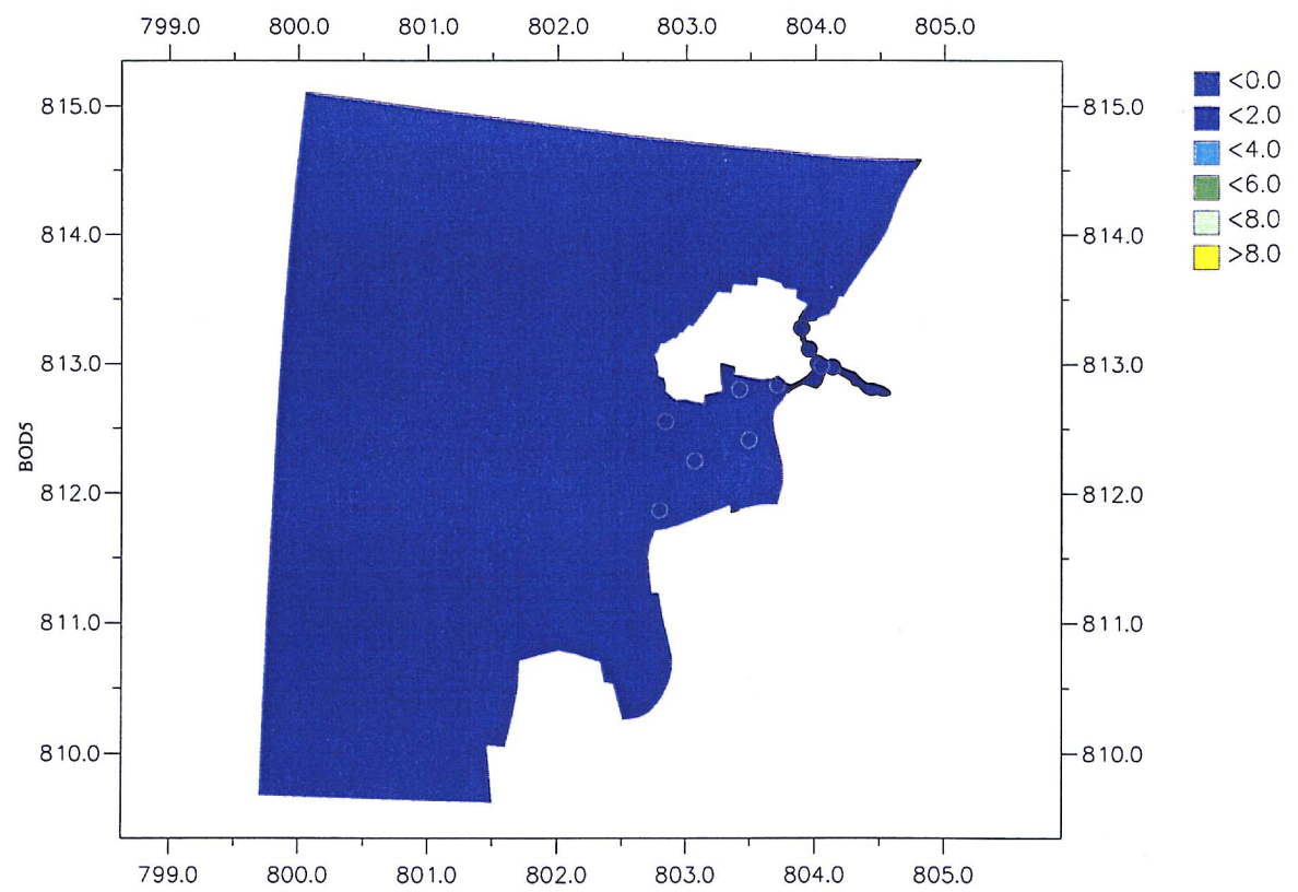
Surface Layer BOD; Dry Season; High Water Upper – Fine Grid Regional Model; Lower – Tai O Detailed Model Dots at Tai O Bay – Tai O Boat Anchorage Field Data
