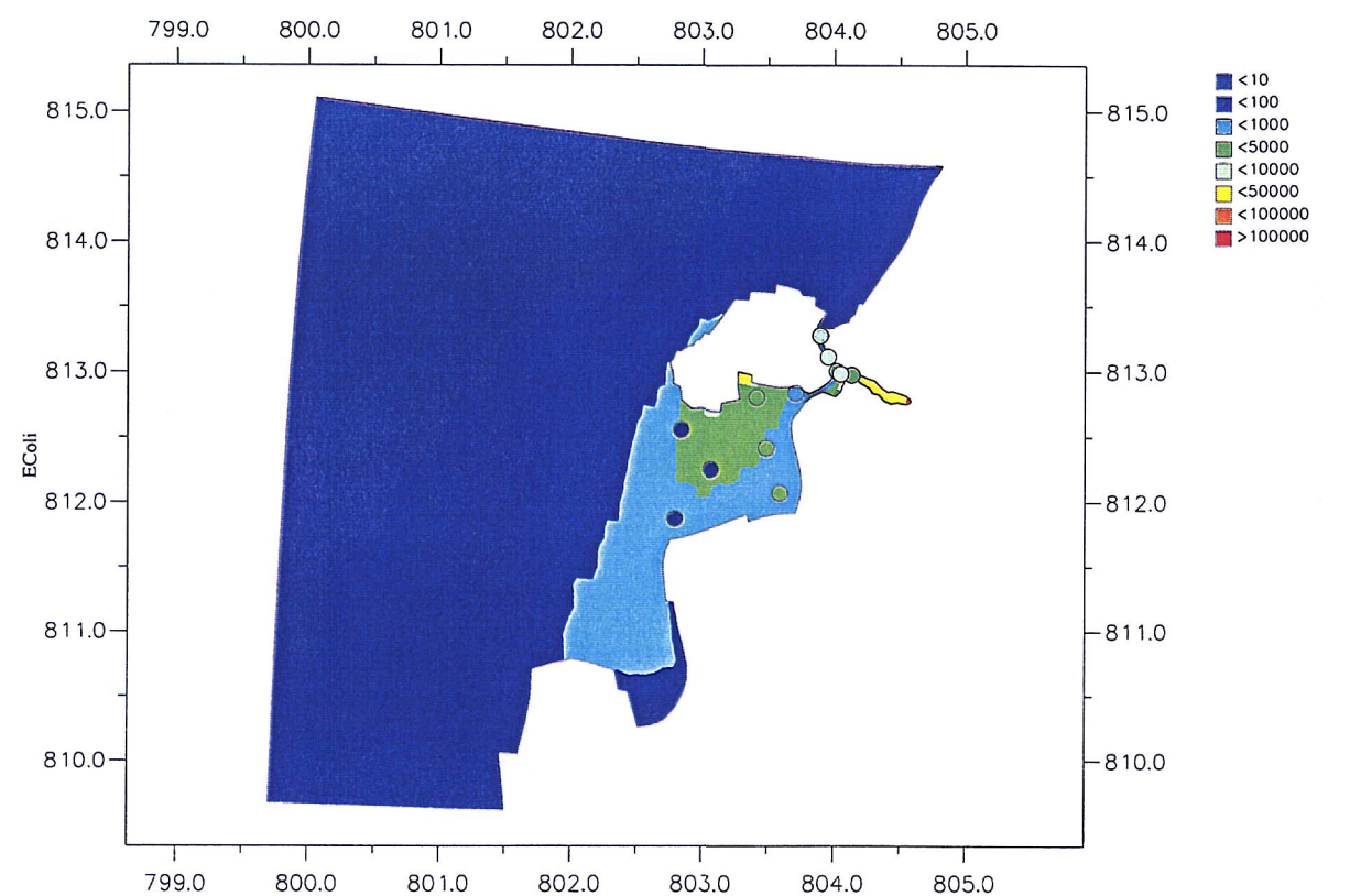
Surface Layer E. Coli; Dry Season; Low Water Upper – Fine Grid Regional Model; Lower – Tai O Detailed Model Dots at Tai O Bay – Tai O Boat Anchorage Field Data
