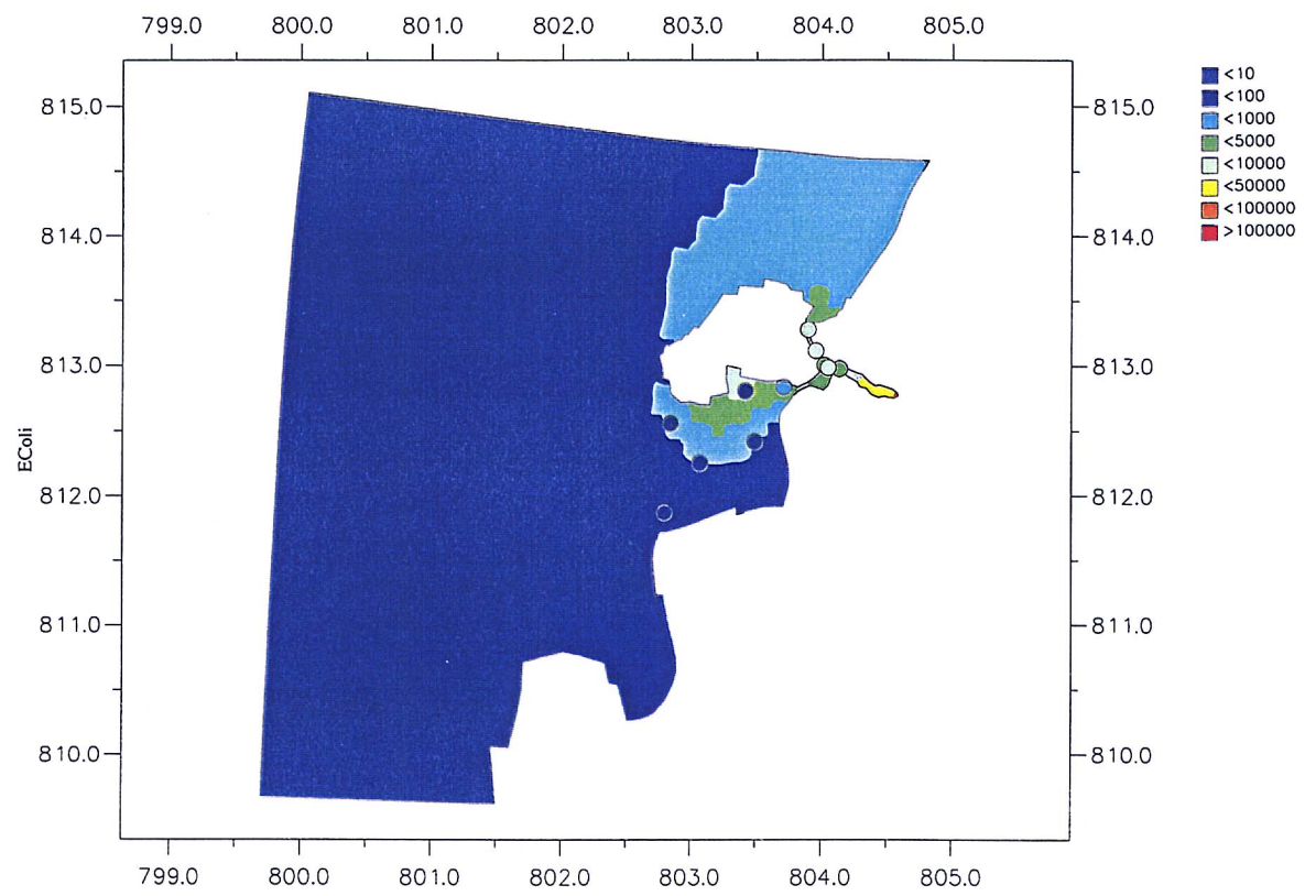
Surface Layer E. Coli; Dry Season; High Water Upper – Fine Grid Regional Model; Lower – Tai O Detailed Model Dots at Tai O Bay – Tai O Boat Anchorage Field Data
