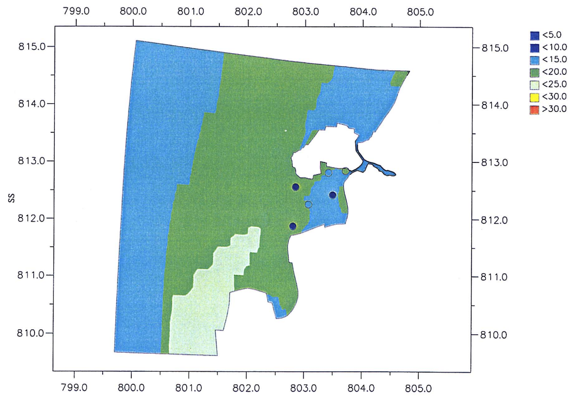
Surface Layer Suspended Solids; Dry Season; High Water Upper - Fine Grid Regional Model; Lower - Tai O Detailed Model Dots - Tai O Boat Anchorage Field Data
