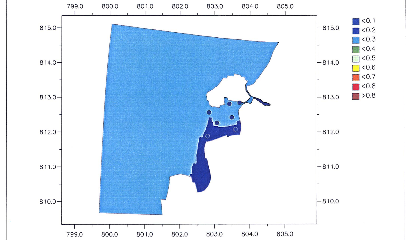
Surface Layer Total Inorganic Nitrogen; Dry Season; Low Water Upper - Fine Grid Regional Model; Lower - Tai O Detailed Model Dots - Tai O Boat Anchorage Field Data
