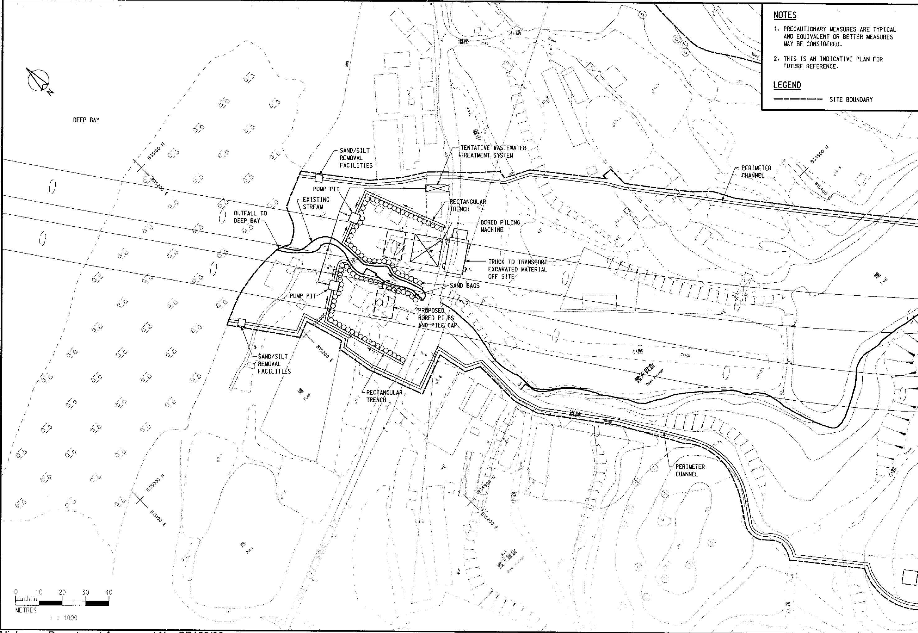
Figure 4.3 Precautionary Drainage Measures during Bored Pile Construction - Plan
