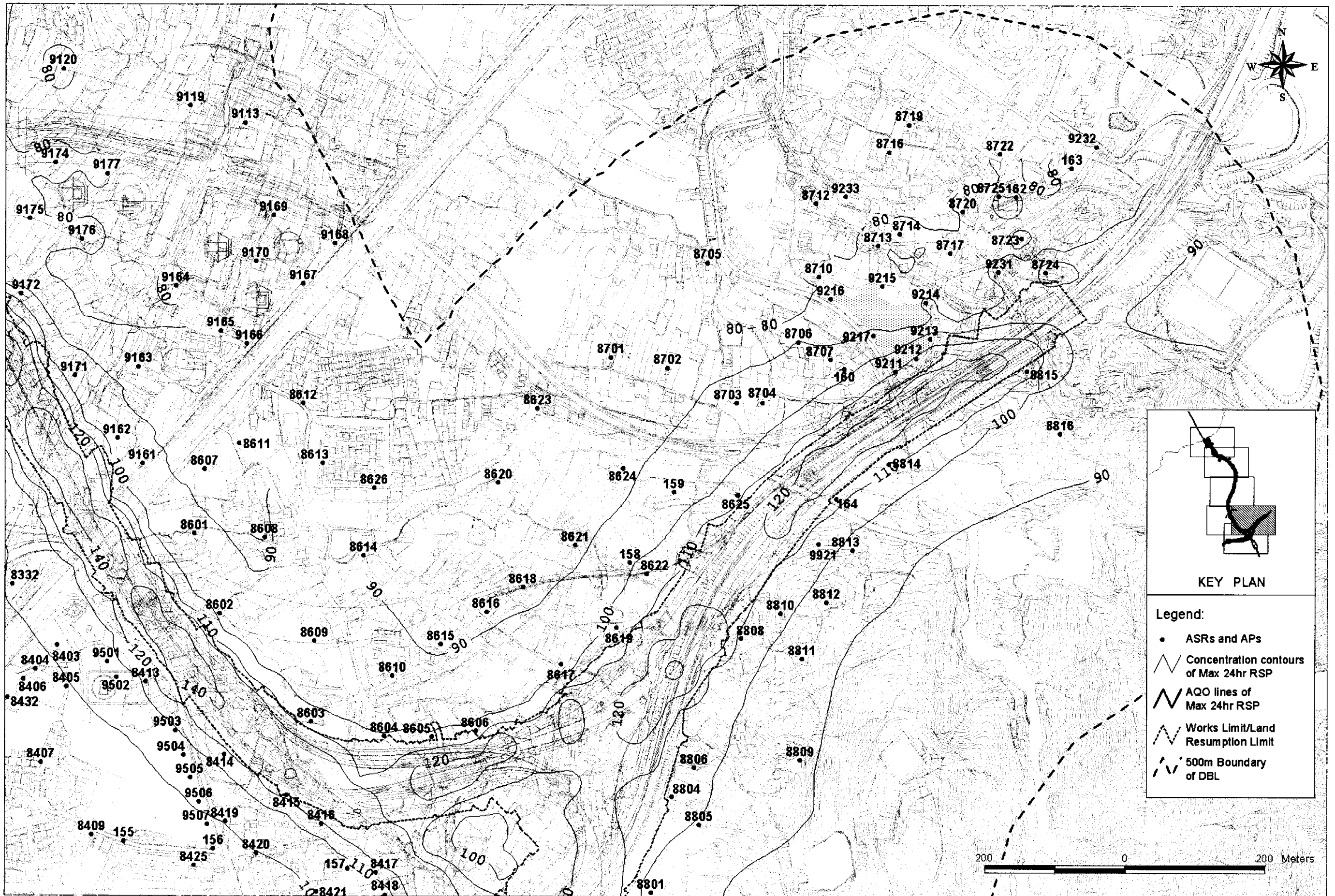
Figure 2.7E Concentration Contours of Predicted Worst-case 24-hour Average Respirable Suspended Particulates Level at 10m Above Ground
