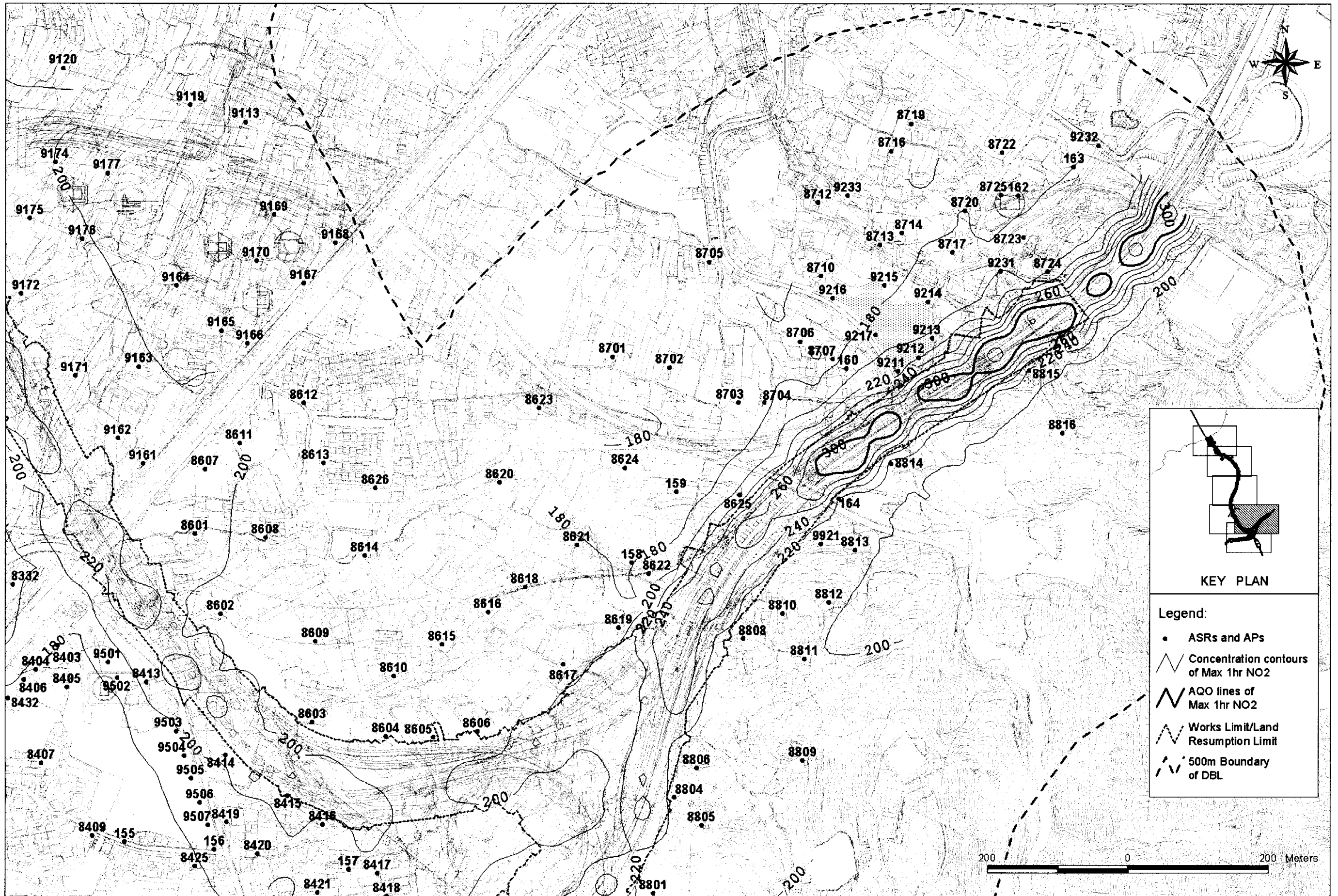
Figure 2.2E Concentration Contours of Predicted Worst-case 1-hour Average Nitrogen Dioxide Level at 1.5m Above Ground
