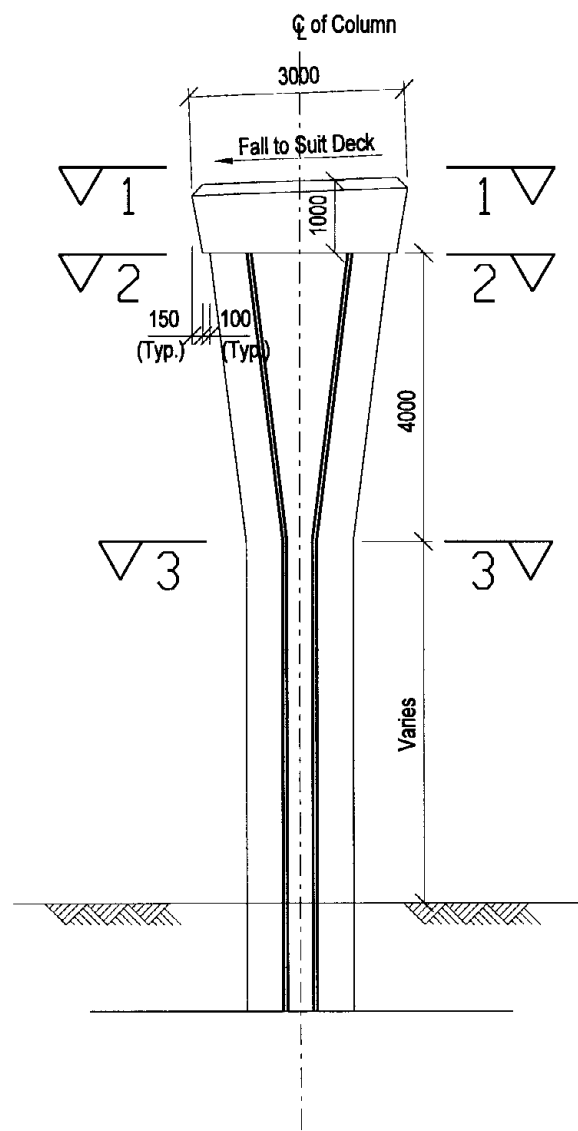
TYPE A COLUMN
