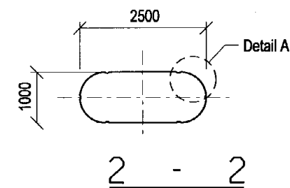
ELEVATION FOR COLUMN HEAD AT BRIDGE MOVEMENT JOINT
