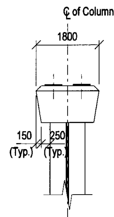
ELEVATION FOR COLUMN HEAD AT BRIDGE MOVEMENT JOINT
