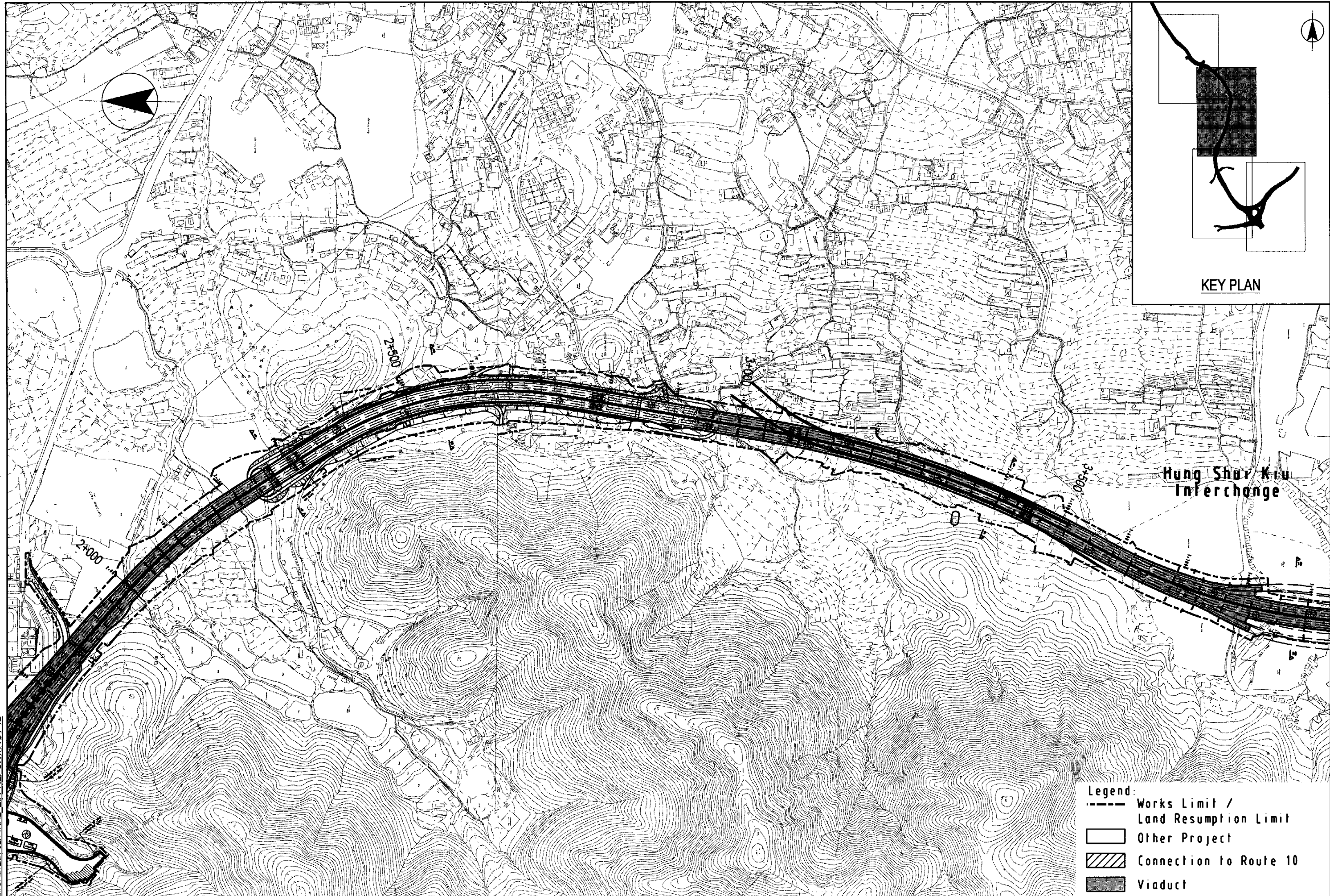
Figure 1.1B Deep Bay Link General Layout Plan
