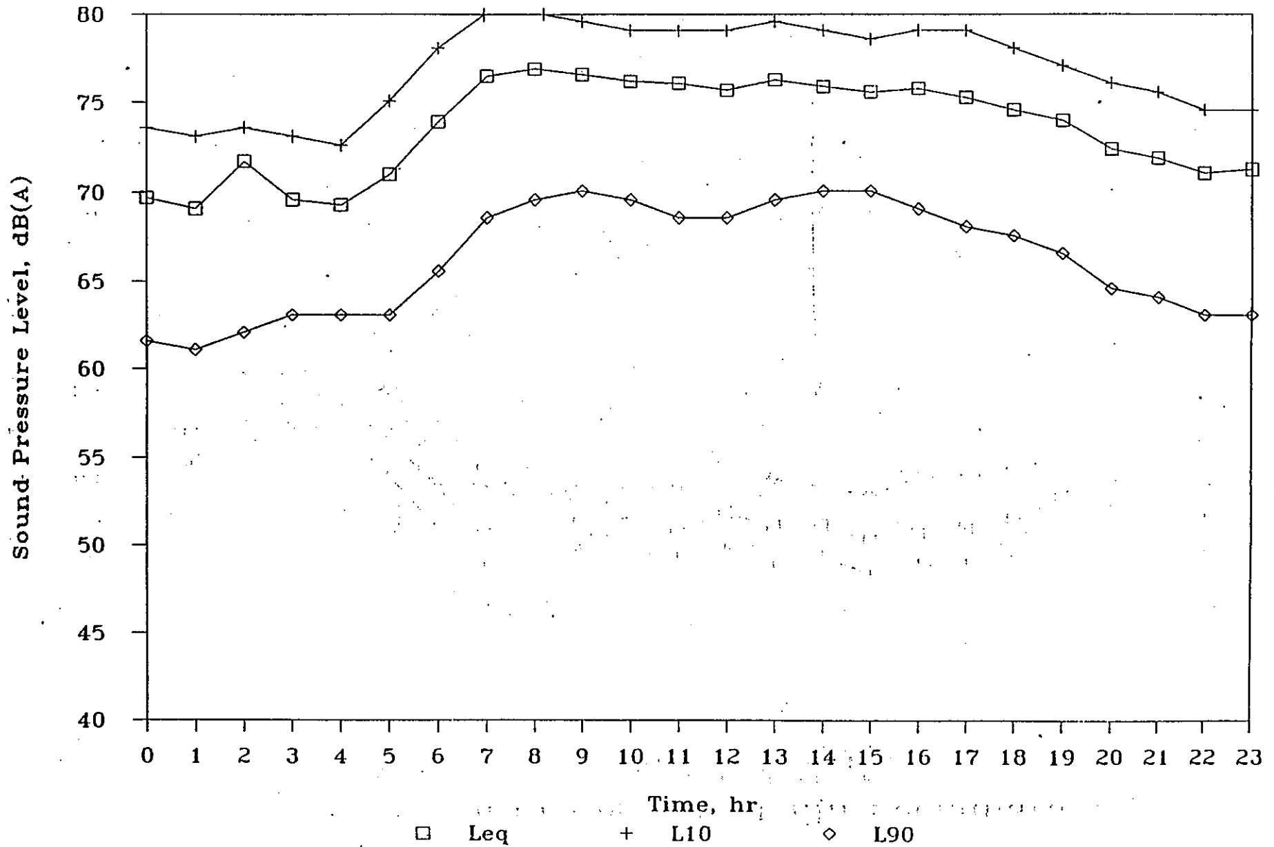
Figure 2j Noise Monitoring - West Kln Reclamation
