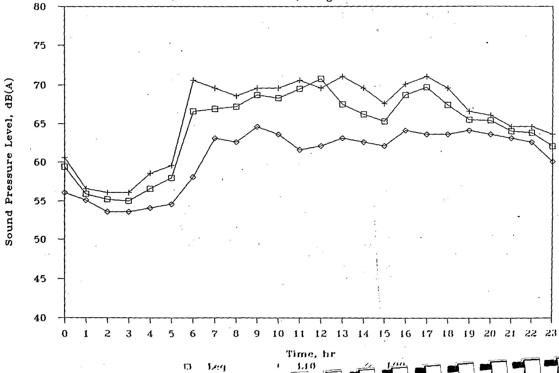
Figure 2f Noise Monitoring - West Kln Reclamation
