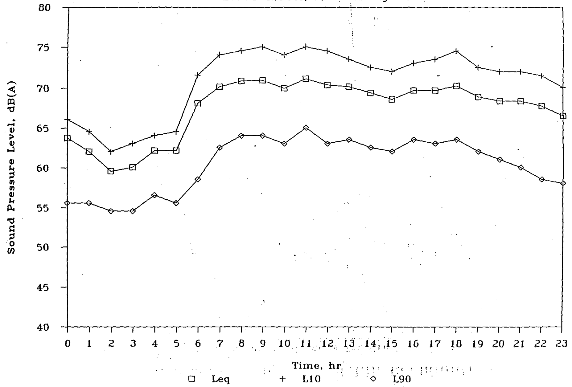
Figure 2g Noise Monitoring - West Kln Reclamation
