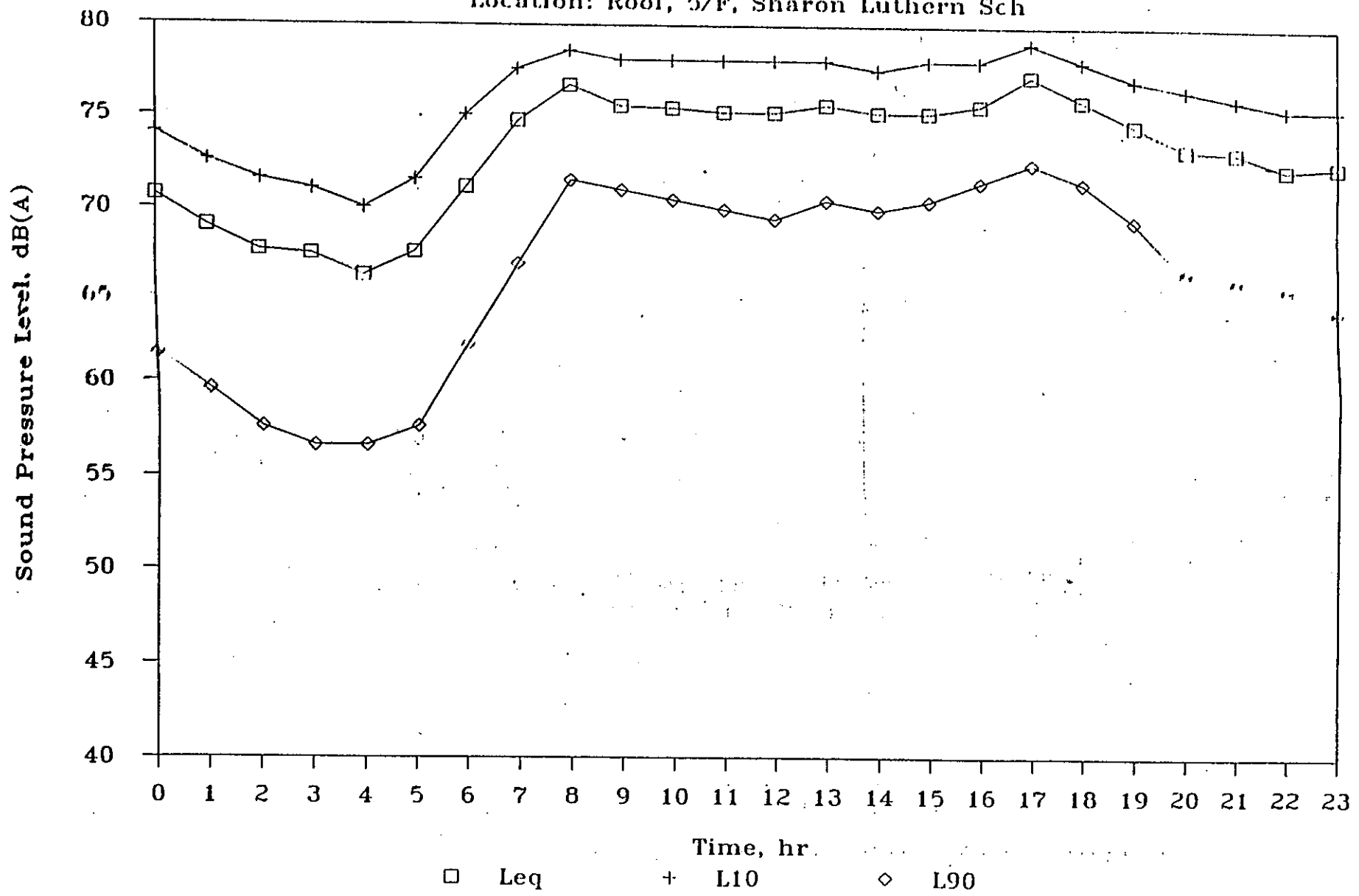
Figure 2h Noise Monitoring - West Kln Reclamation
