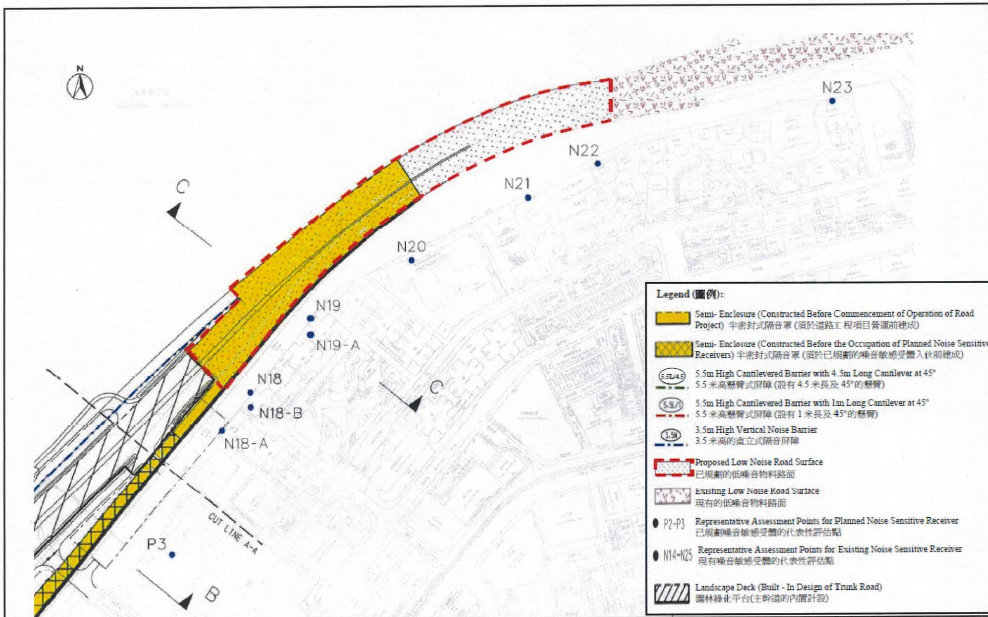
Figure 2b: Locations of Direct Noise Mitigation Measures (Sheet 2 of 3) 圖 2b : 直接噪音緩解措施位置圖 (第2張, 共3張)
