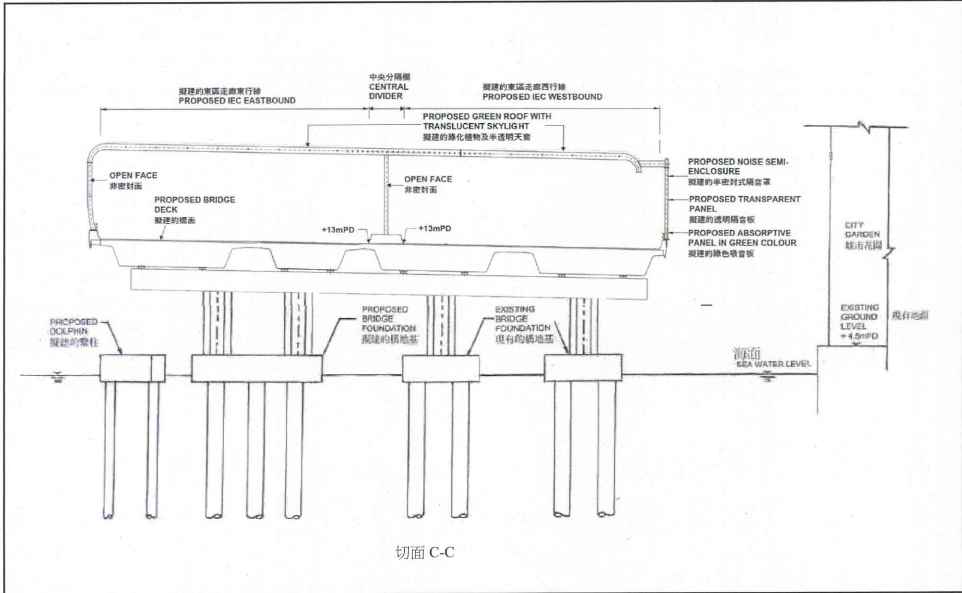
Figure 2f: Section of Direct Noise Mitigation Measures 圖 2f: 直接噪音緩解措施切面圖
