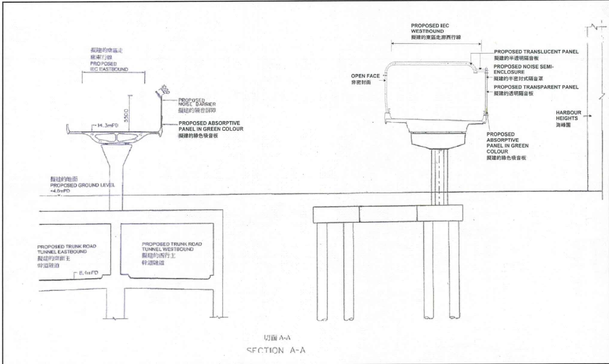
Figure 2d: Section of Direct Noise Mitigation Measures 圖 2d : 直接噪音緩解措施切面圖
