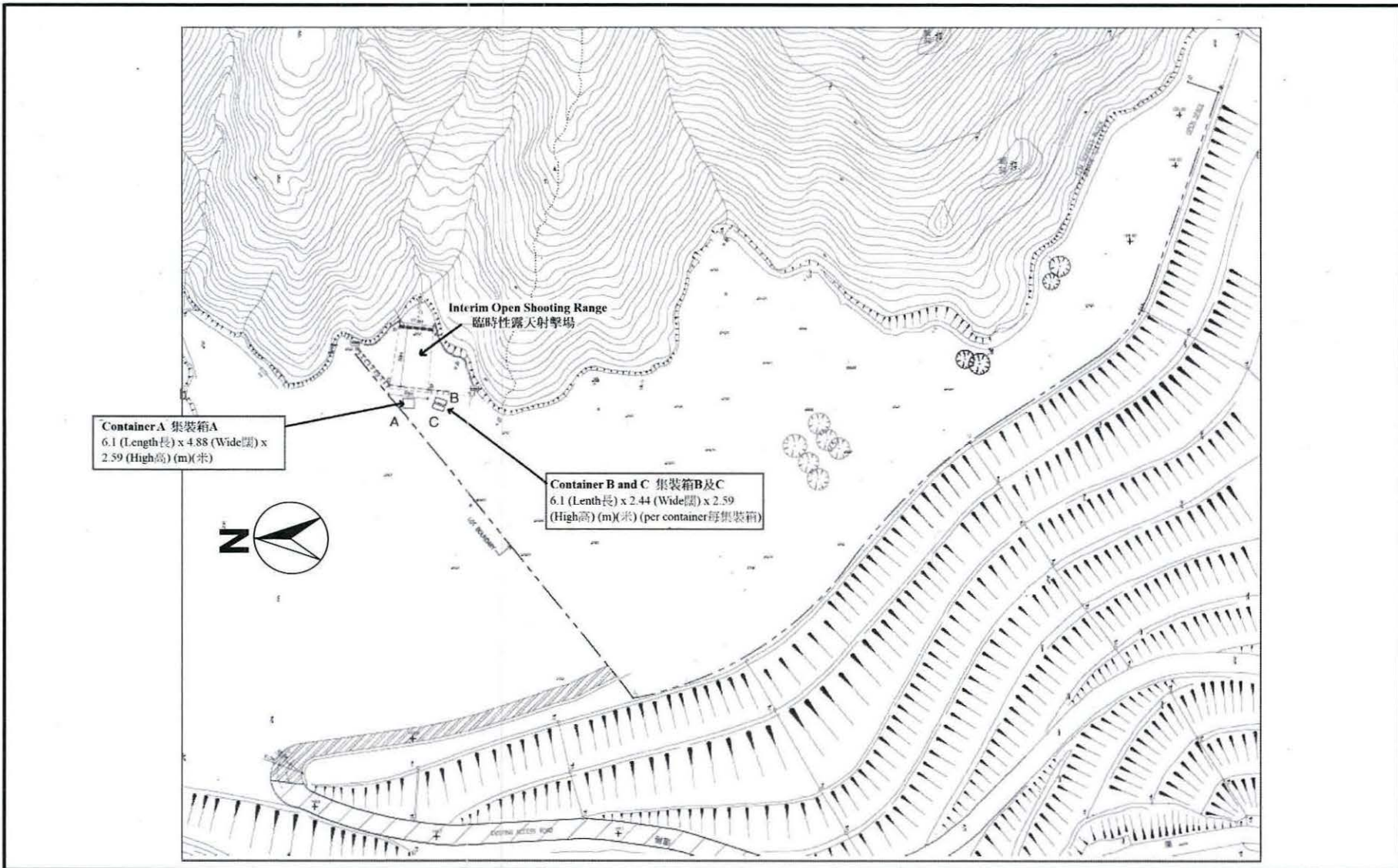
Figure 2 - Layout Plan of the Interim Open Shooting Range
