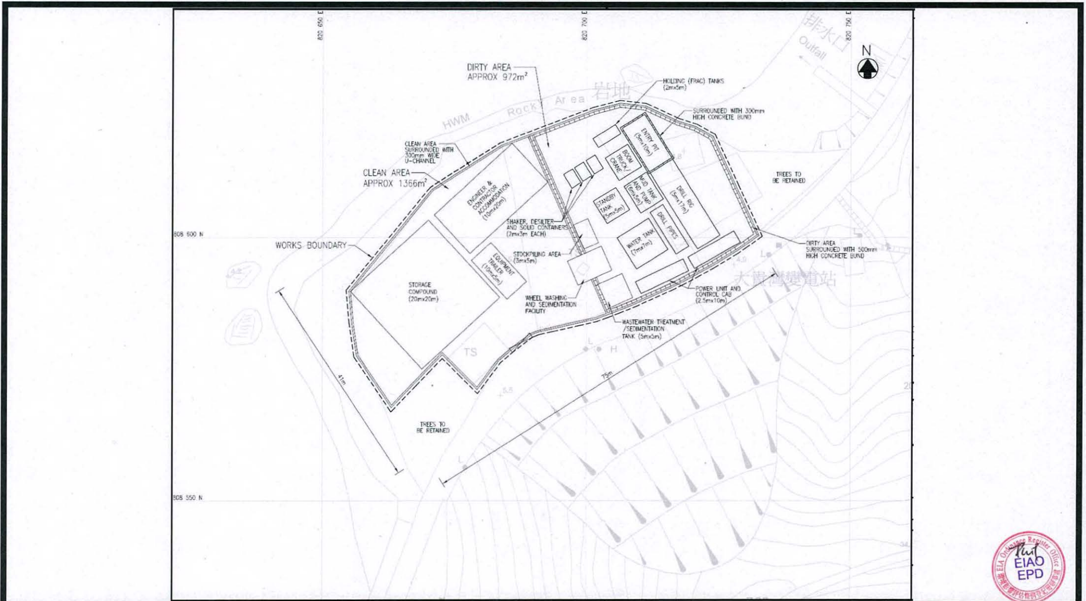
Figure 4: Schematic Layout of Drainage Measures at Cheung Chau Works Area
