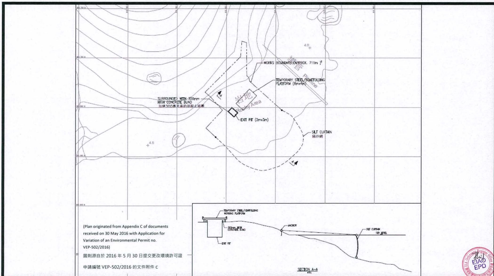
Figure 5: Schematic Layout and Silt Curtain Installation at Lantau Works Area
