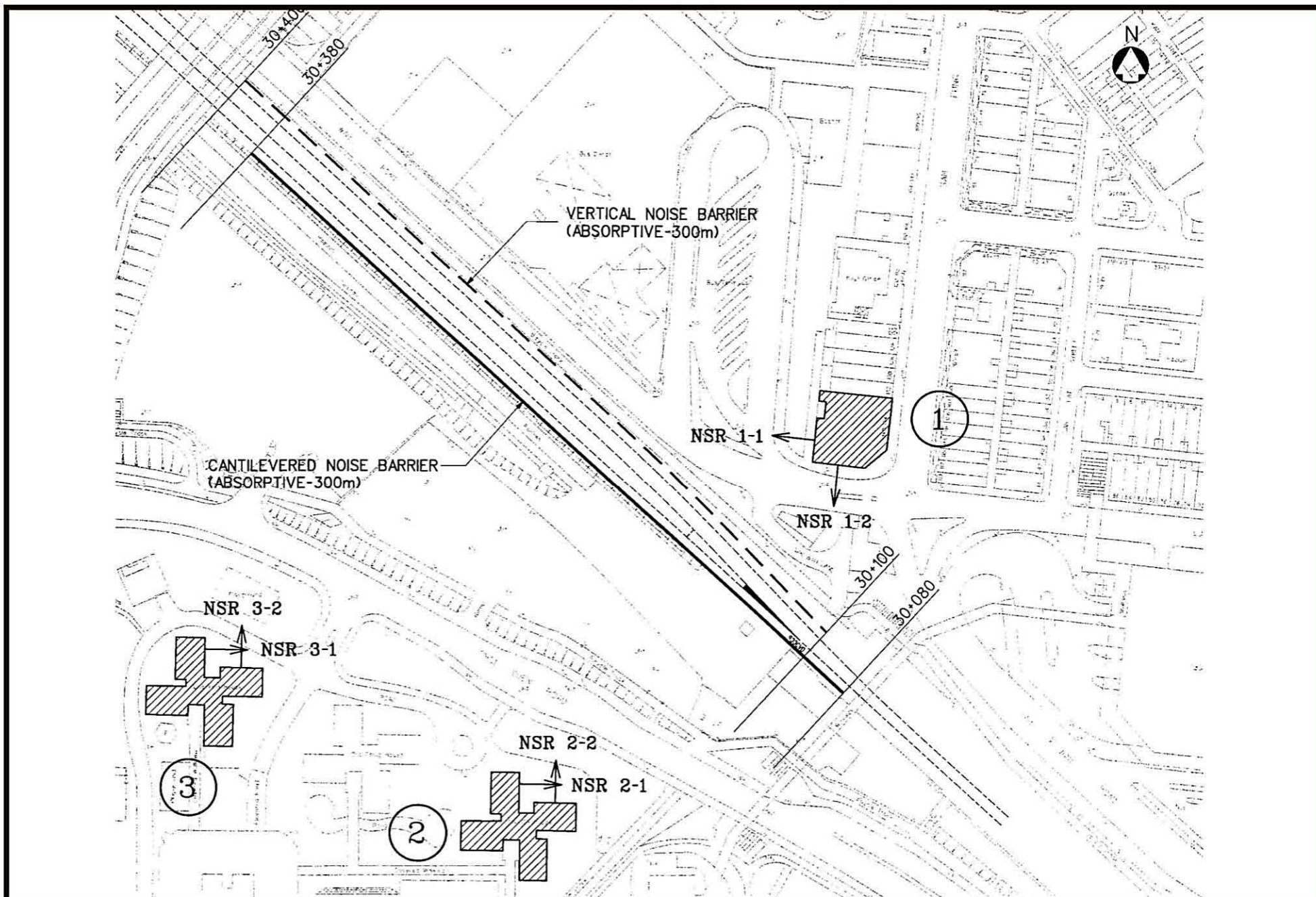
Figure 9 - Sheung Shui to Lok Ma Chau Spur Line (上水至落馬洲支線) Locations of Noise Barriers as described in Condition 3.27 of the Permit 圖九 - 條例 3.27 所指之隔音屏障位置 Reproduced from Drawing No. 7.2b (Volume 5 of 5) of the EIA Report (Register number AEIAR-052/2002) 摘自環評報告第五冊圖 7.2b (登記冊編號 AEIAR-052/2002)
