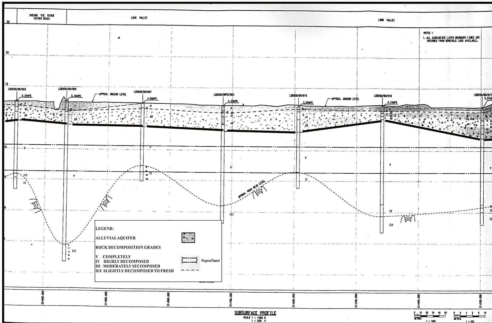
Sheung Shui to Lok Ma Chau Spur Line (上水至落馬洲支線) Figure 3 - The vertical profile of the tunnel across Long Valley as described Condition 3.12 圖三 - 條例3.12所指貫穿塱原之隧道垂直側面圖 (Reproduced from Figure 1 of Appendix A3.1 (Volume 3 of 5) of the EIA Report (Register No.: AEIAR-052/2002) 摘自環評報告第三冊附件A3.1圖一 (登記冊編號:AEIAR-052/2002)
