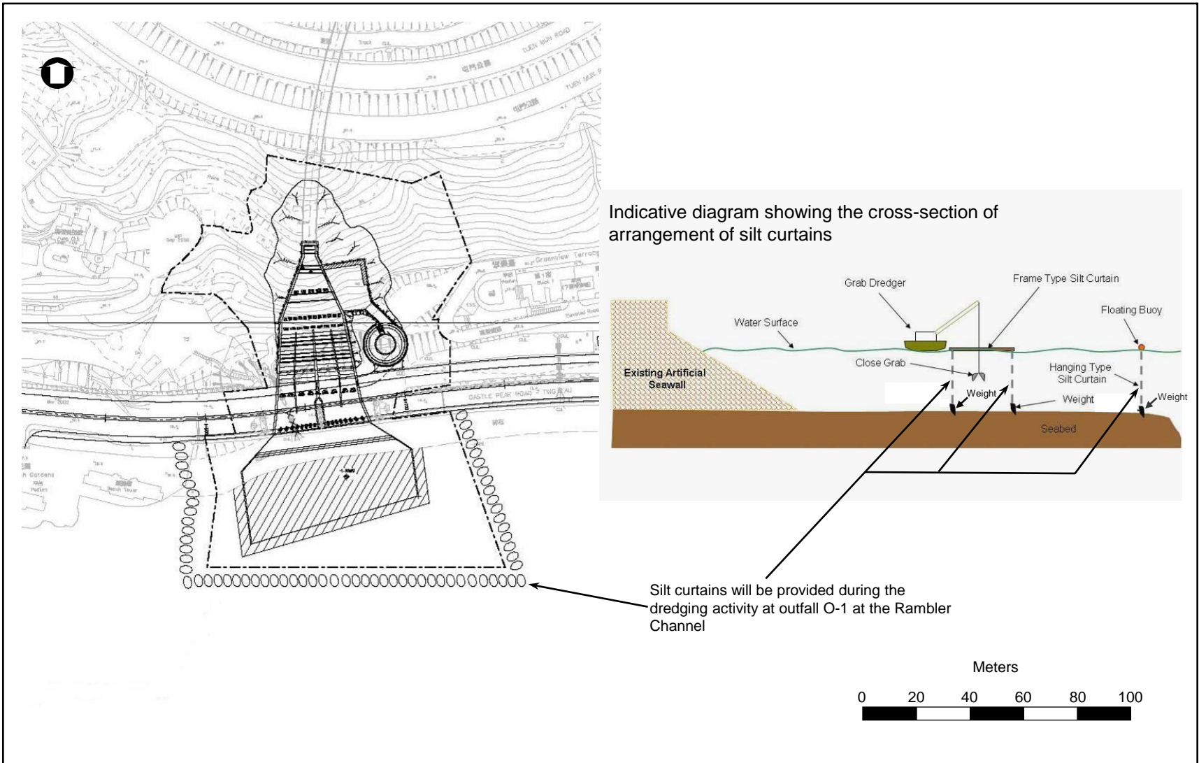
Figure 9 : Indicative Arrangement of Silt Curtains at Outfall O-1 圖 9 : 於出水口O-1而設的淤泥屏障安排示意圖
