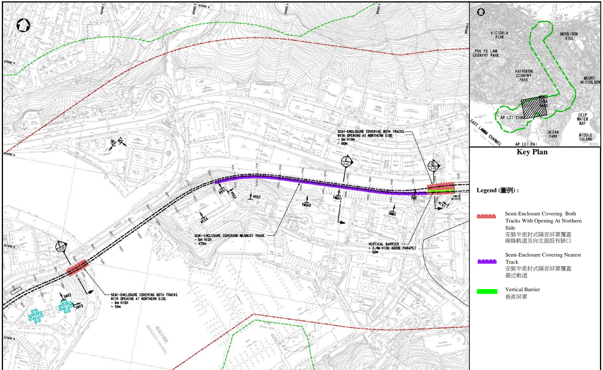
Figure 13: Mitigation Measures for Noise Operational Air-Borne Noise 圖 13: 營辦期間的空氣傳導噪音緩解措施
