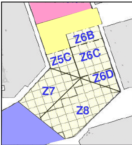
Dredging Rate Requirements for Dredger Operating in Zones Z5C, Z6B, Z6C, Z6D, Z7 & Z8
