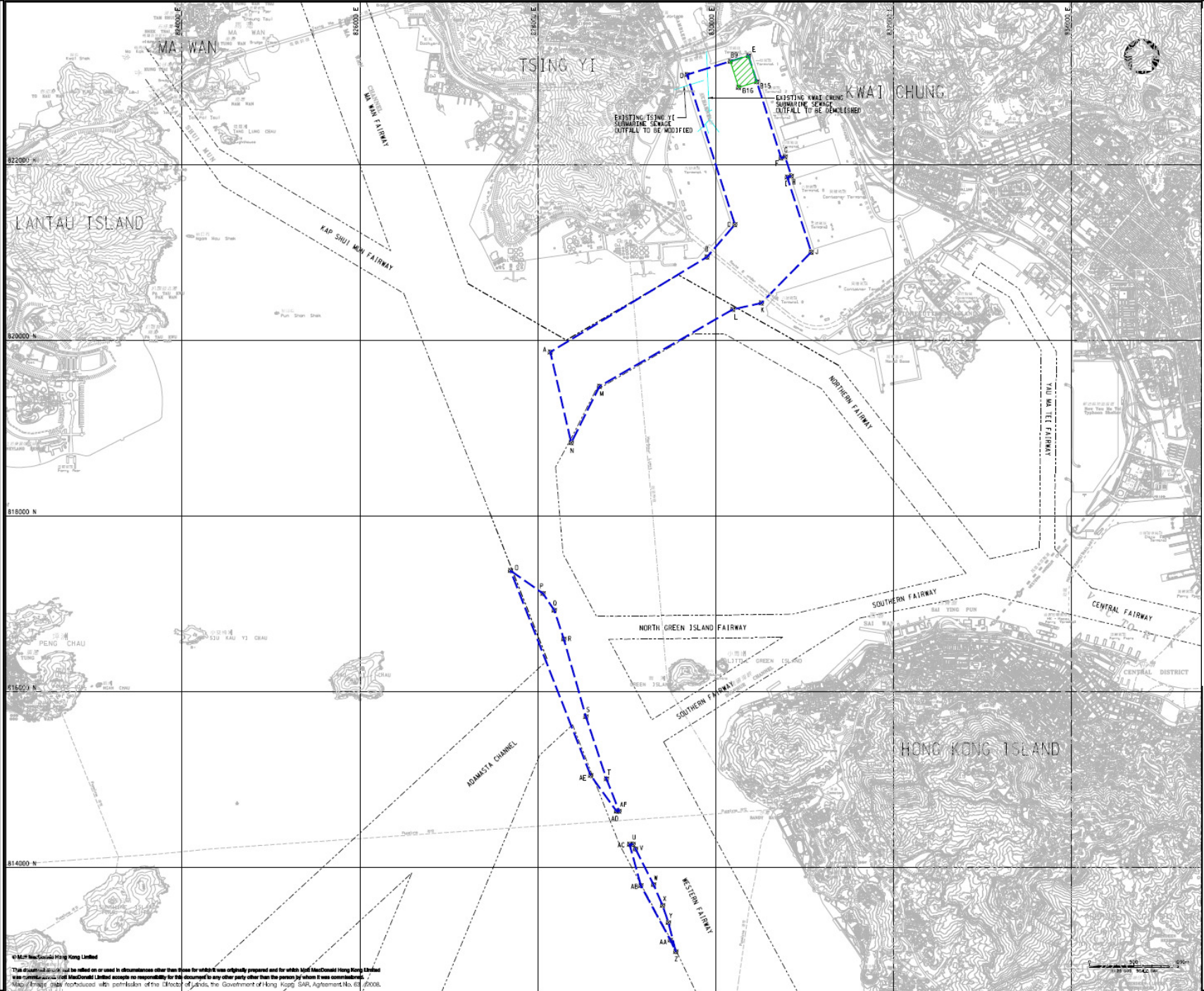
Project Title: Providing Sufficient Water Depth for Kwai Tsing Container Basin and its Approach Channel Figure 1: Project Layout (Extracted from Figure 1 of Justification for the Proposed Demarcation of the Dredging Zones)
