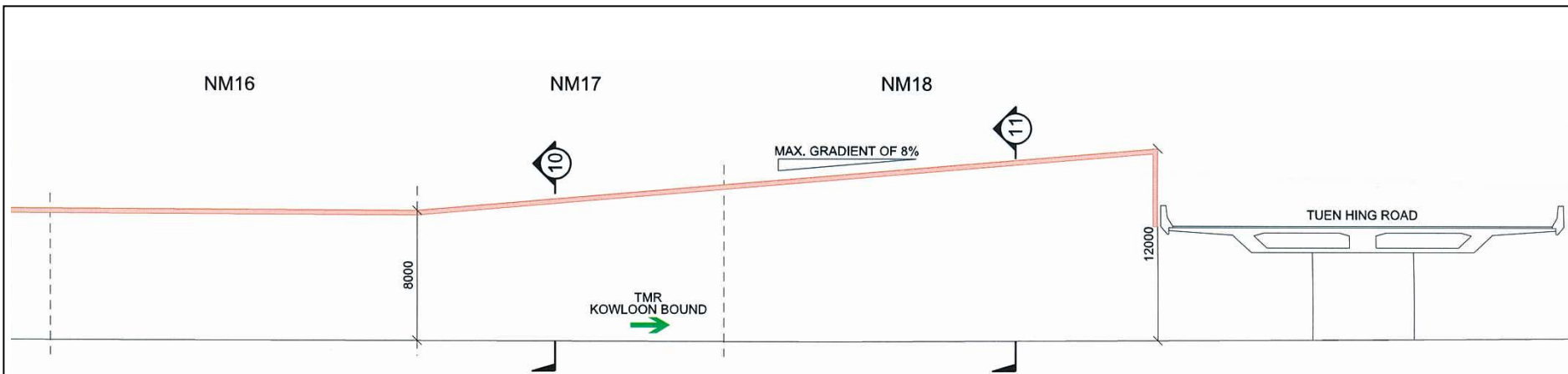
LONGITUDINAL SECTION ALONG TMR KOWLOON BOUND BETWEEN NM16 - NM18 (N.T.S.)
