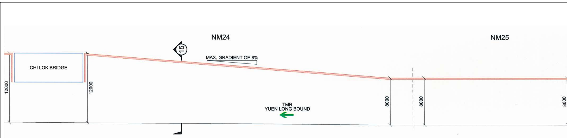
LONGITUDINAL SECTION ALONG TMR YUEN LONG BOUND BETWEEN NM24 AND NM25 (N.T.S.)
