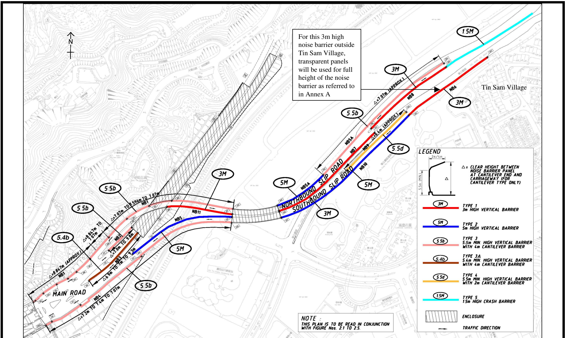
Figure 2 Noise Barriers and Enclosures (Extracted from the Application VEP-238/2007)
