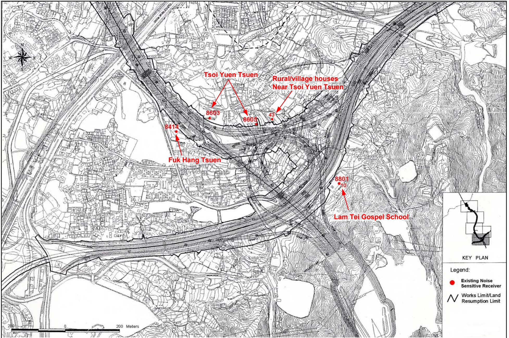
Deep Bay Link and Widening of Yuen Long Highway between Lam Tei and Shap Pat Heung Interchange (Lam Tei to Tan Kwai Tsuen Section) -
