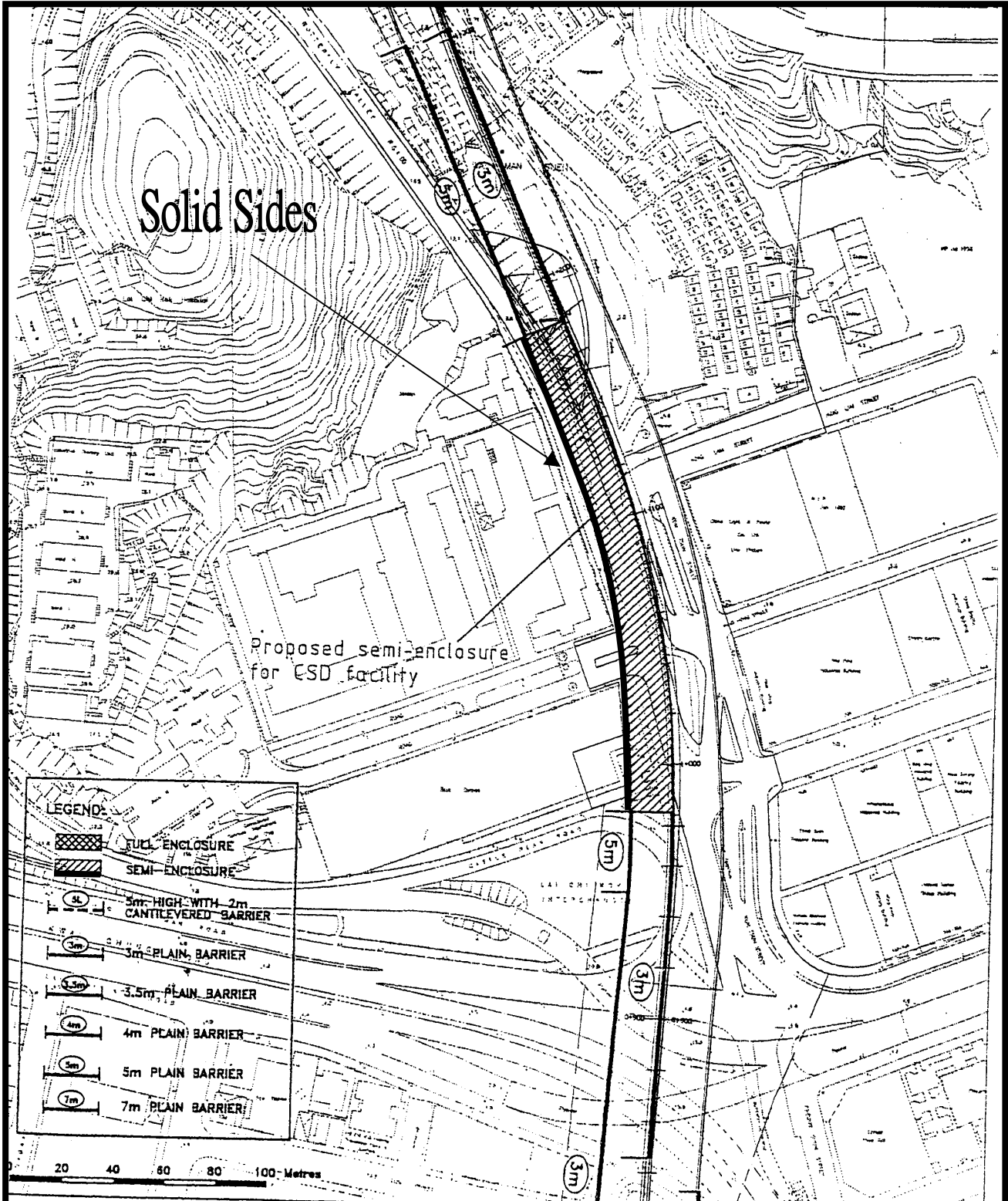
Figure 3 Noise Barriers and Enclosures (Extracted from the Application VEP-180/2005)
