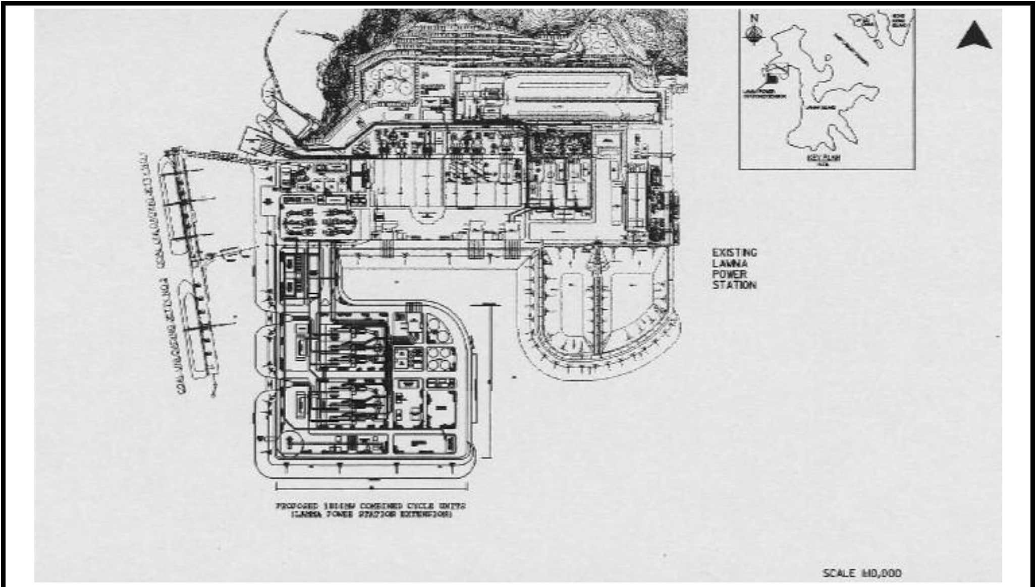
Figure A1: The Location of 1,800MW Gas-fired Combined Cycle Plant at the Lamma Extension Site (Ref. Figure 4.4b, Part B in Vol. 1 of the EIA Report)
