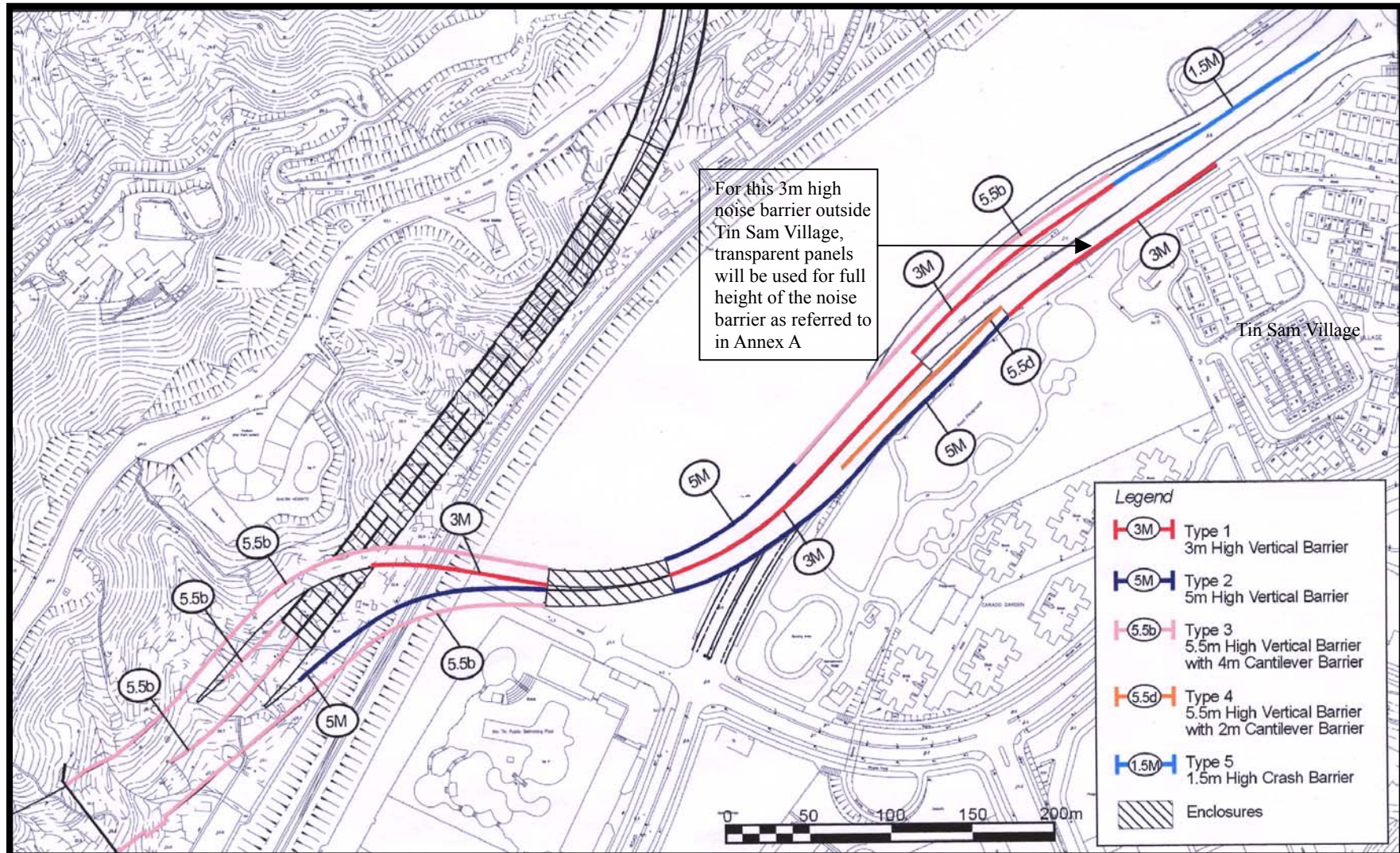
Figure 2 Noise Barriers and Enclosures (Extracted from the Application VEP-163/2005)
