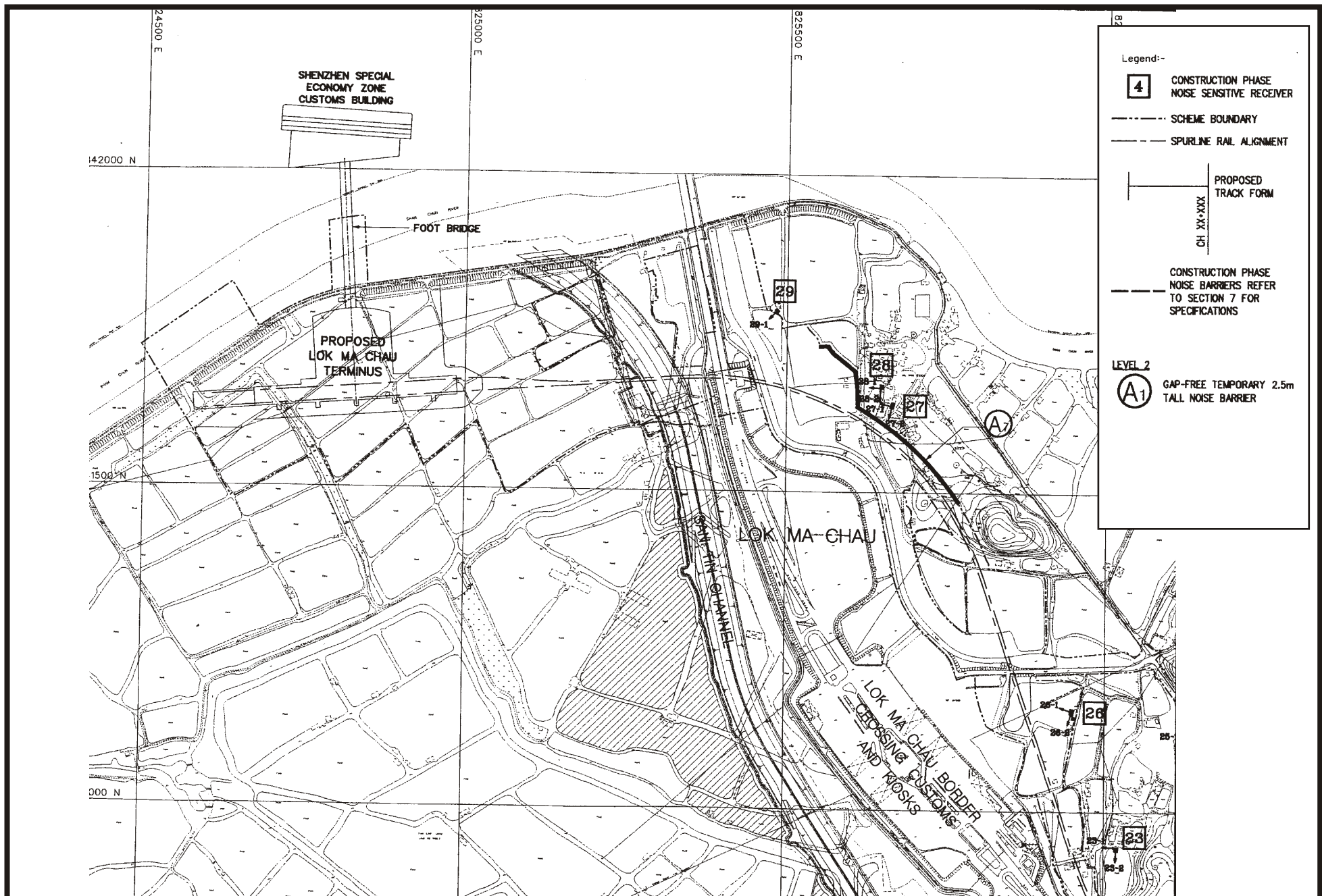
Figure 9e Permit 圖九e - Sheung Shui to Lok Ma Chau Spur Line (上水 至 落馬州 支線) - Locations of Construction Noise Barriers as described in Condition 3.25 of the 條例3.25 所指消除 建築工程 噪音之隔 音屏障位置 Reproduced from Drawing No. 7.1 (Sheet 5 of 5)(Volume 5 of 5) of the EIA Report (Register number AEIAR-
