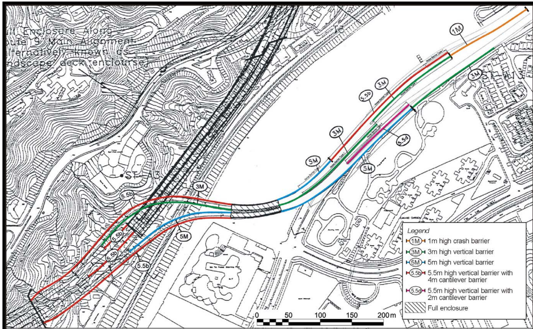
Figure 2 Noise Barriers and Enclosures (Extracted from the Application VEP-124/2003)
