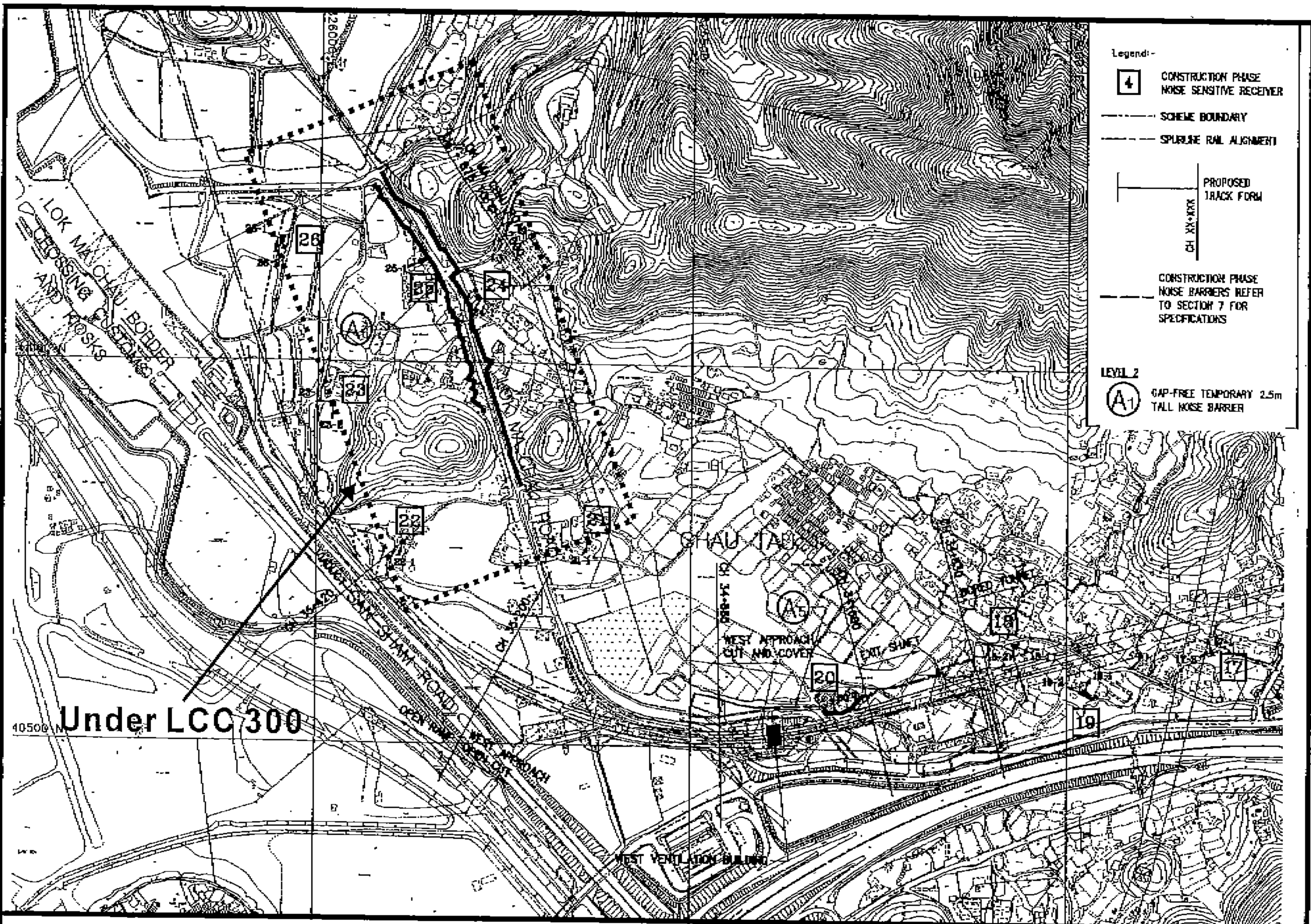
Figure 7d - Locations of Construction Noise Barriers as described in Condition 3.17 of the Permit 圖七丁 - 條例3.17所指消除建築工程噪音之隔音屏障位置 Reproduced from Drawing No. 7.1 (Sheet 4 of 5) (Volume 5 of 5) of the EIA Report (Register number AEIAR-052/2002) 摘自環評報告第五冊圖 7.1 (第四張)(登記冊編號AEIAR-052/2002)
