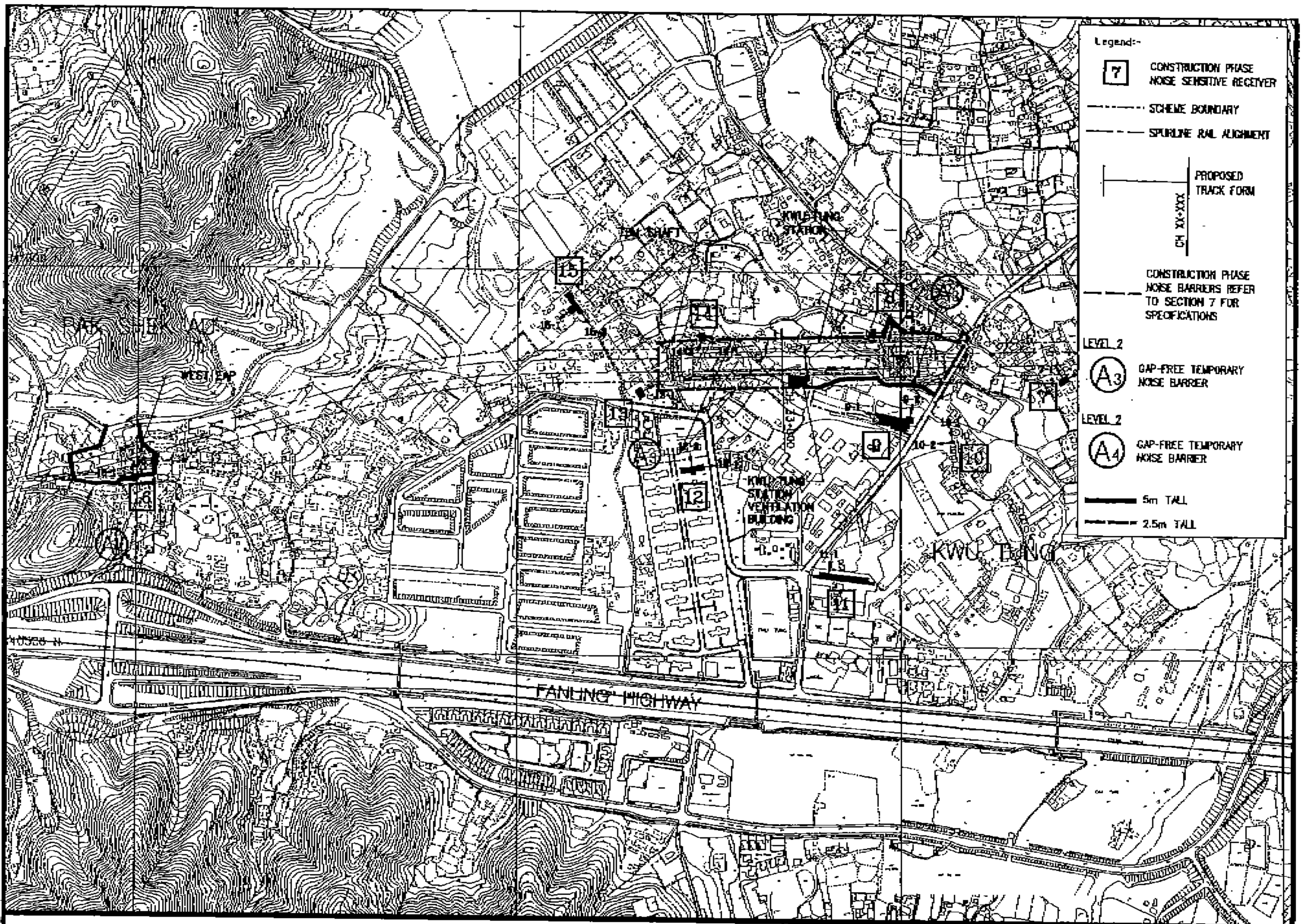
Figure 7c - Locations of Construction Noise Barriers as described in Condition 3.17 of the Permit 圖七丙 - 條例3.17所指消除建築工程噪音之隔音屏障位置 Reproduced from Drawing No. 7.1 (Sheet 3 of 5) (Volume 5 of 5) of the EIA Report (Register number AEIAR-052/2002) 摘自環評報告第五冊圖 7.1 (第三張)(登記冊編號AEIAR-052/2002)
