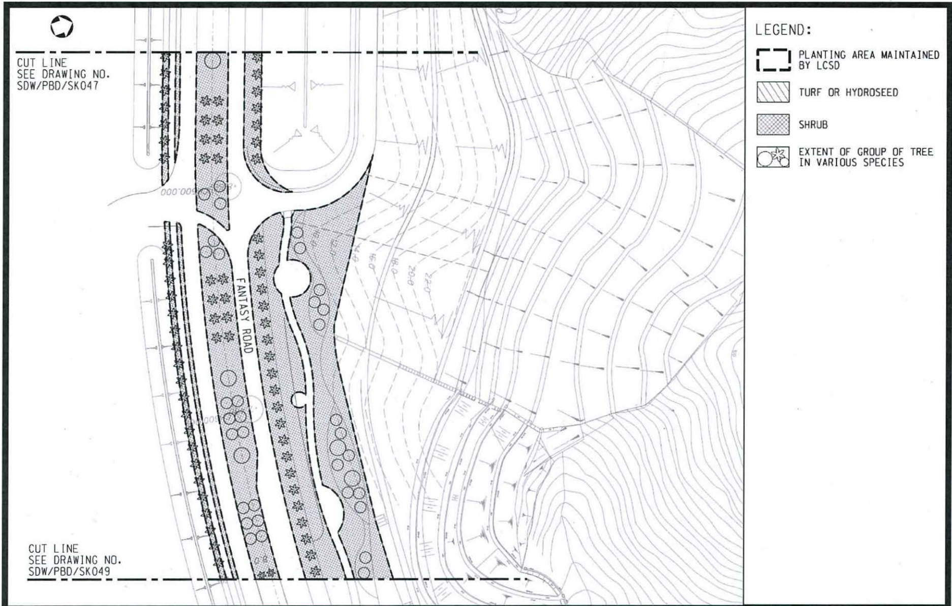
Figure R9: Chok Ko Wan Link Road (Part) Road P2 - Yam O to Penny's Bay (Part) 圖 R9 : 竹篙灣連接路 (部份) P2 公路 - 陰澳至竹篙灣 (部份)
