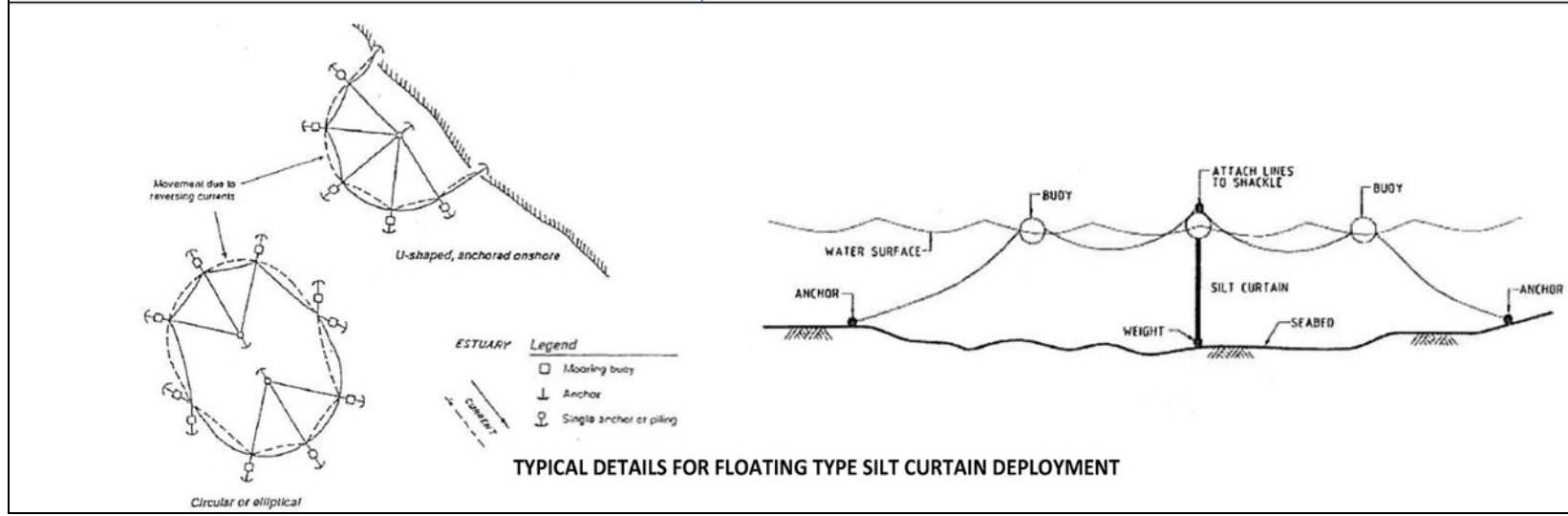
Figure 3: Typical Configurations of Silt Curtains and Silt Screens
