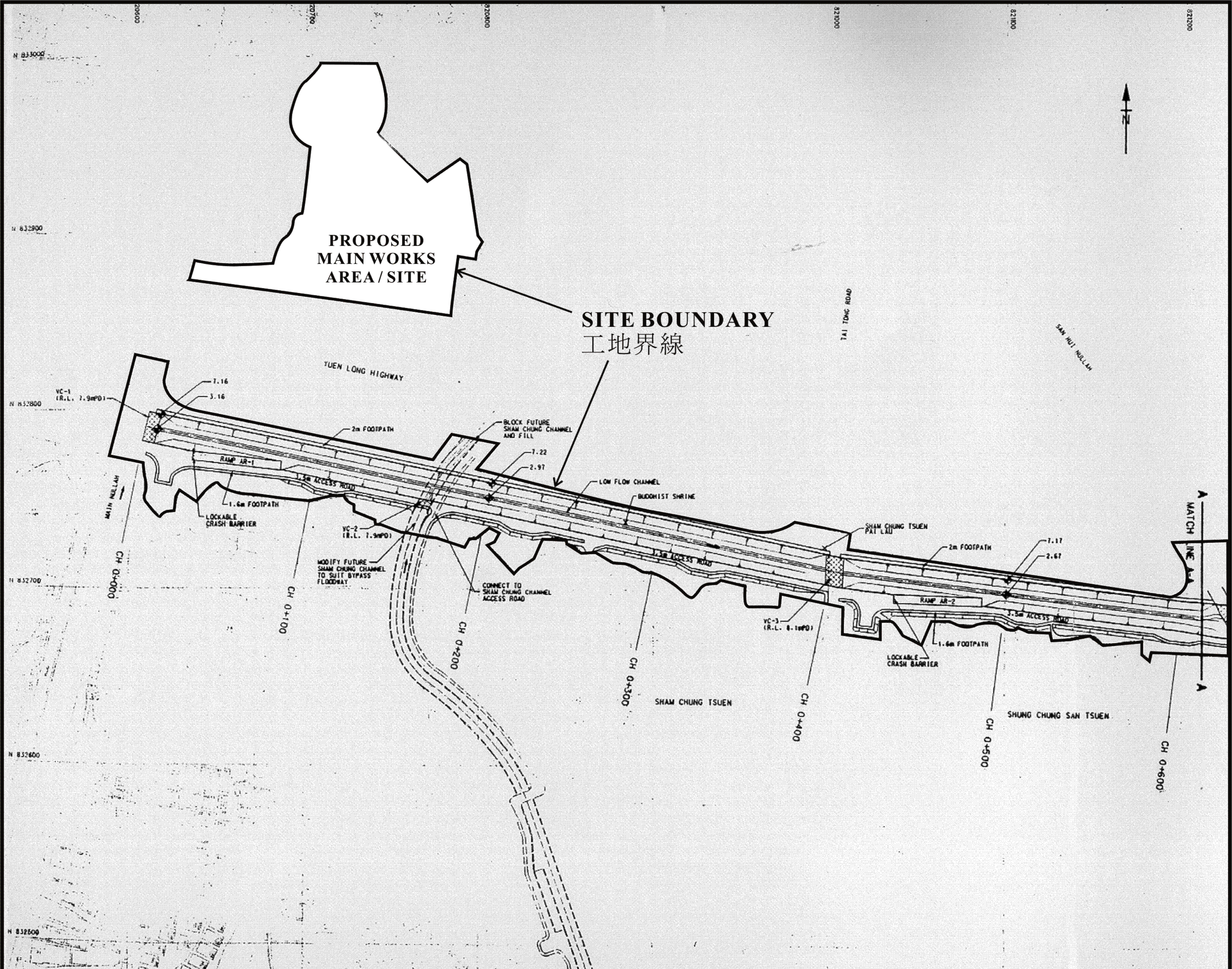
Figure 1.1 Location Plan of Yuen Long Bypass Floodway
