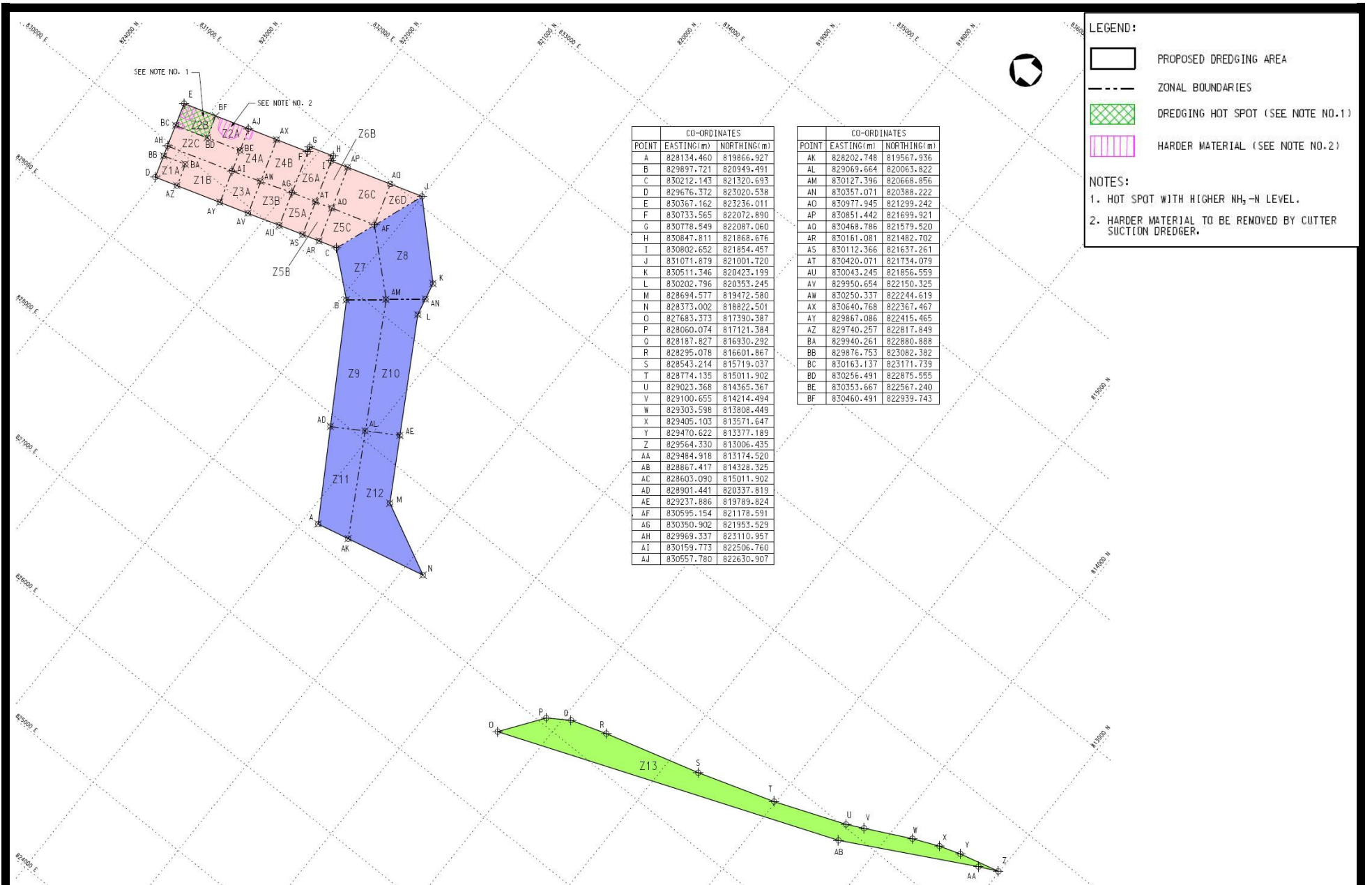
Project Title: Providing Sufficient Water Depth for Kwai Tsing Container Basin and its Approach Channel Figure 2: Zones and Sub-zone of Dredging Plan Layout (Extracted from Figure 1.2h of the EM&A manual)
