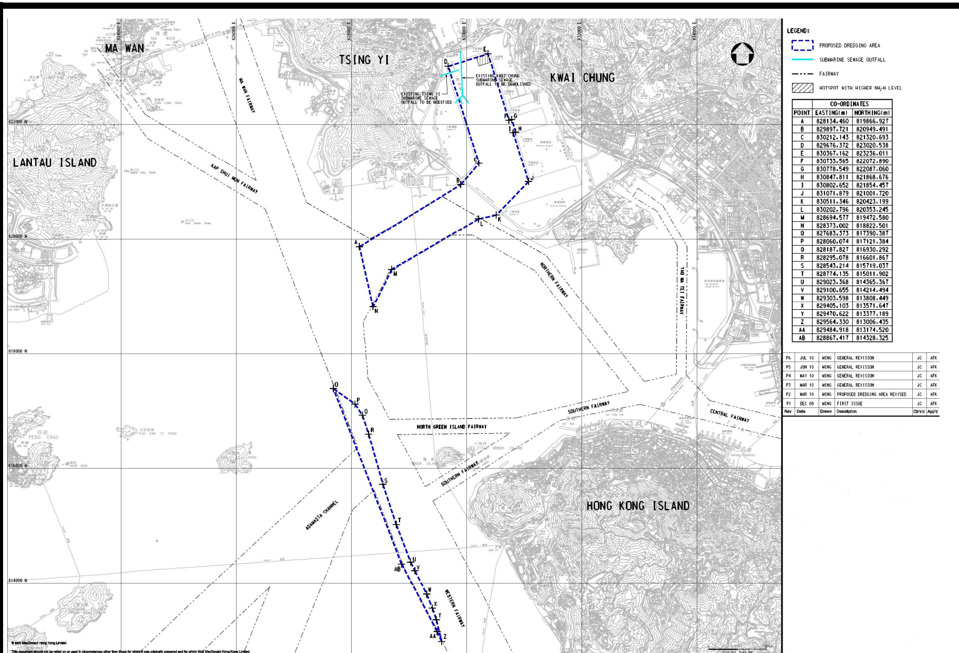
Project Title: Providing Sufficient Water Depth for Kwai Tsing Container Basin and its Approach Channel Figure 1: Project Layout (Extracted from Figure 2.1 of the EP Application)
