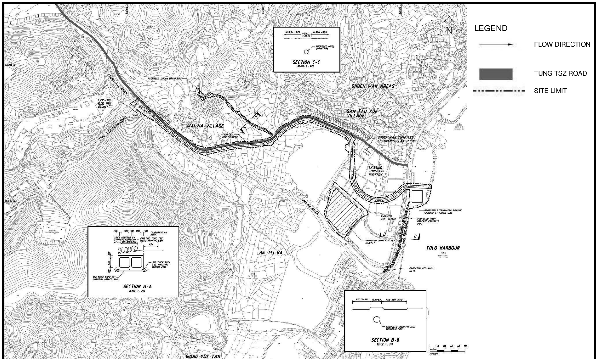
Figure 1 Drainage Improvement Works in Shuen Wan - Location Plan
