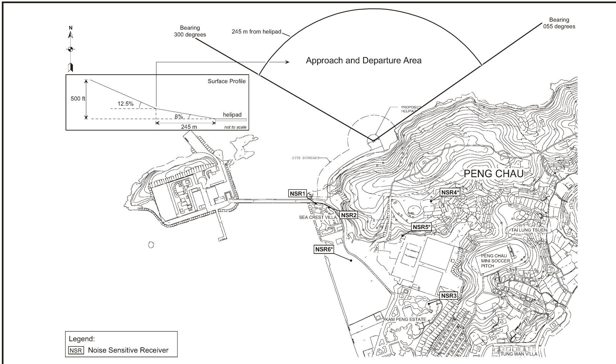
Figure 2 - Helicopter Flight Envelope
