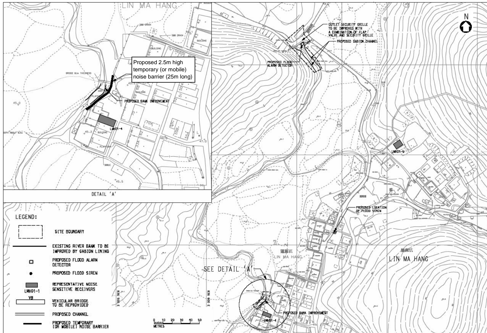
Figure 7 Locations of Temporary Noise Barrier – Lin Ma Hang (LMH01) (Sheet 1 of 2)
