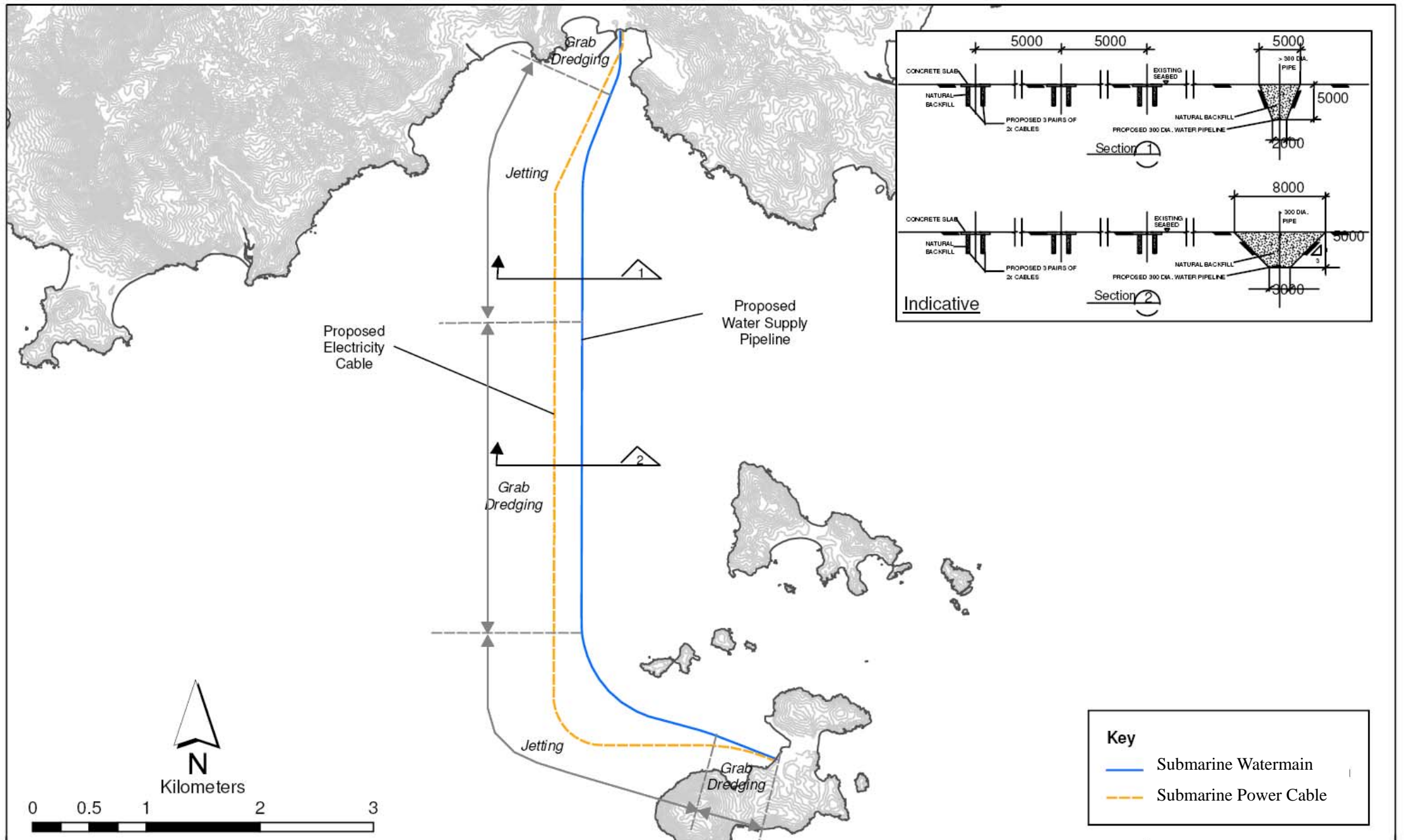
South Soko Island Proposed Water Supply and Electricity Cable Trench Details
