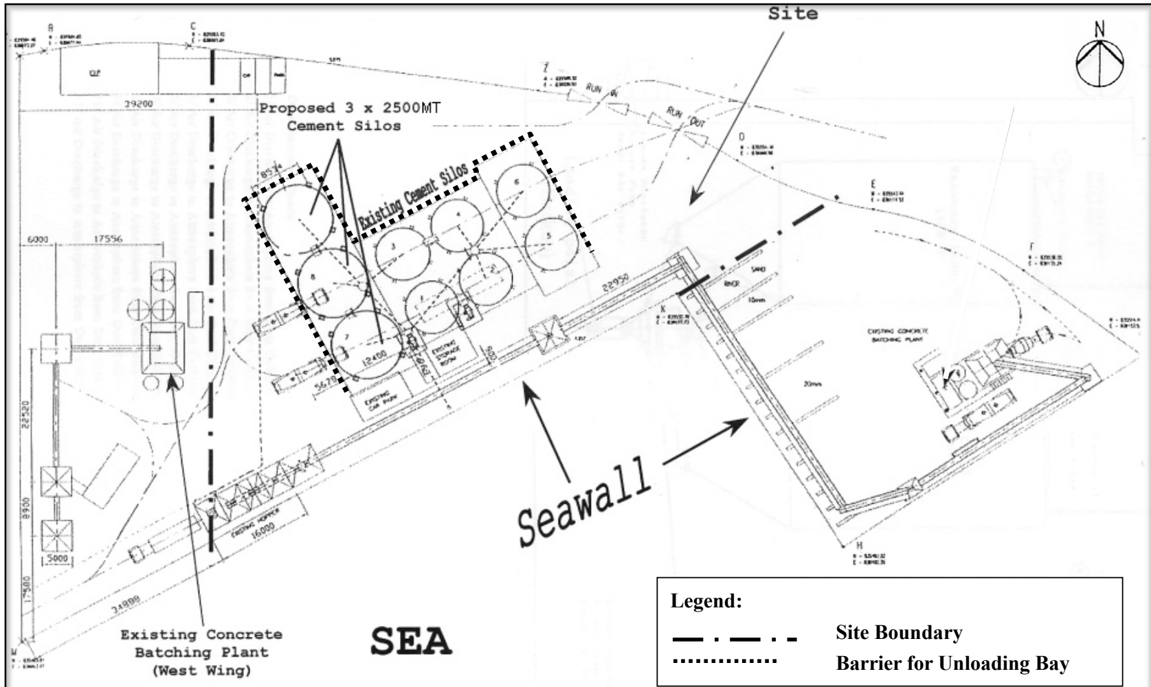
Figure 3 Noise Barriers at the Cement Silos (Modified from Figure 5.5 of the EIA Report)
