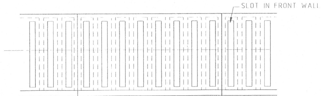
FRONT ELEVATION OF CAISSON
